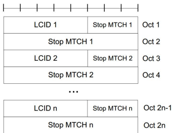
Fig. 3: MSI MAC control Element (3GPP TS36.321)
