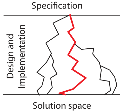
Fig. B.1: The task of designing and implementing an algorithm can be seen as going from a specification to a solution. Typical more than one solution will satisfy the same specification. However, when constraints are introduced, the solution space narrows down and only a few or one “implementation tracks” (depicted as the thick red line) will result in a satisfying solution.
