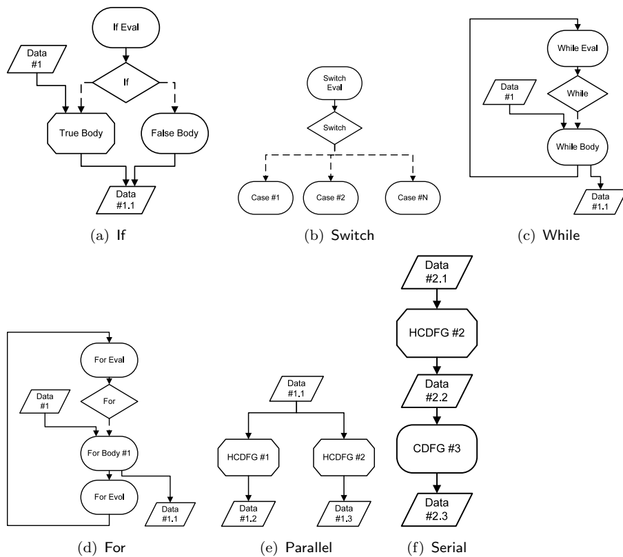
Fig. A.4: Overview of the different CFGs and combined HCDFGs, on which the cyclomatic complexity values are measured. Between the (HC)DFGs there is a set of data exchange nodes which are here left out for simplicity. The symbols are similar to those presented in Fig A.3.
