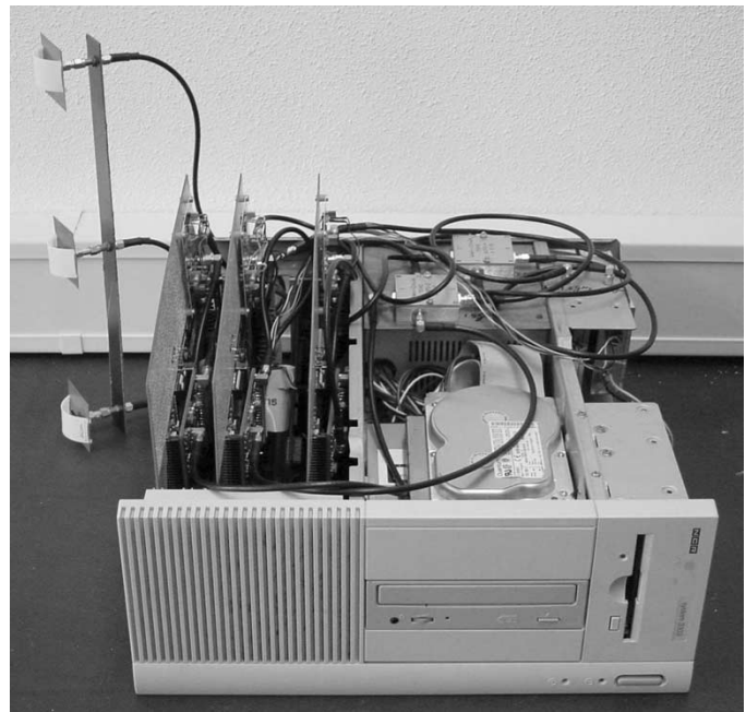
Fig. 7. Receiver equipment: PC with three receiver boards (i.e., the three receiver branches).
