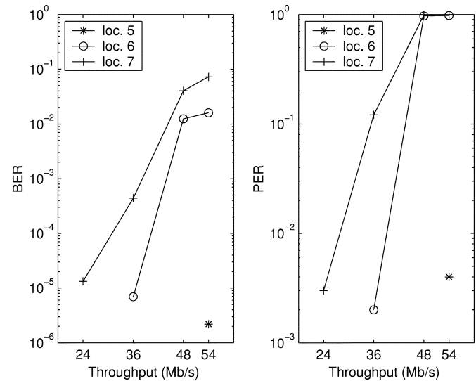
Fig. 11. Measurement results of a 1 \times 1 system with PAC V-BLAST detection for the TX locations 5, 6, and 7.
