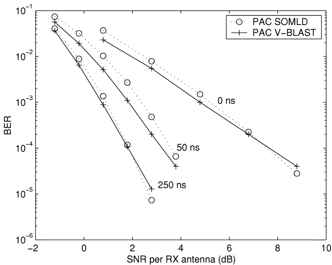
Fig. 6. BER performance for 4 \times 4 PAC schemes, BPSK, rate 1/2 coding, and frequency-selective Rayleigh fading with an exponential decaying PDP with different rms delay spreads.
