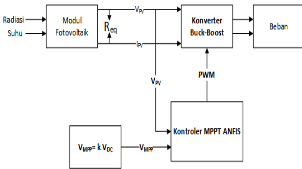
Fig. 8. Block diagram of ANFIS MPPT.
