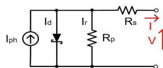
Fig. 1. Single-diode model of photovoltaic cell including parallel and series resistances. [4].
