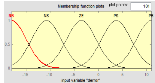
Figure 11. Membership function for input (change error)
