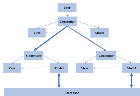
Fig 4: Hierarchical Model View Controller Pattern
