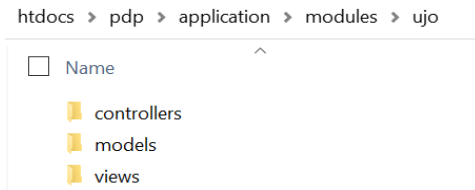
Fig 7.b: Ujo Folder
