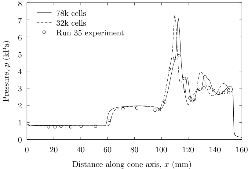
Figure 9: Surface pressure for the 25°-55° biconic, Run 35 configuration.
