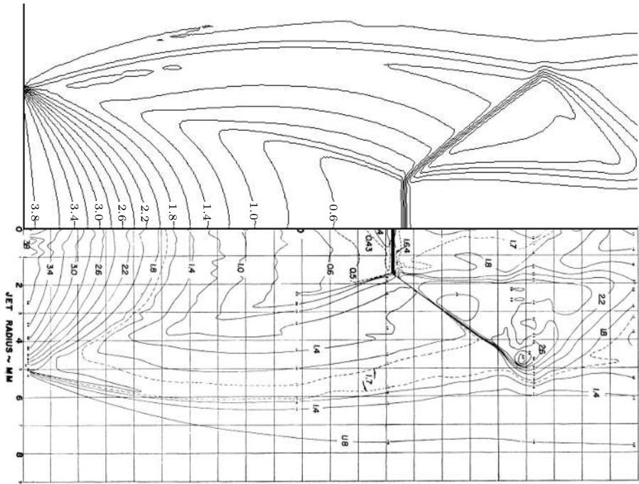
Figure 7: Density contours in the Ladenburg jet; our simulation (top) and original experimental data (bottom).
