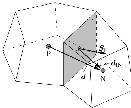
Figure 1: Finite volume discretisation.
