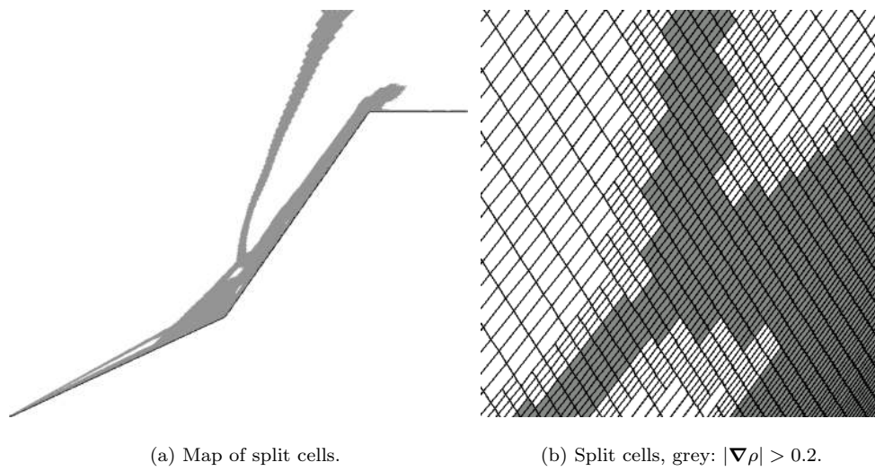
Figure 11: Adaptive mesh refinement for the 25°-55° biconic.
