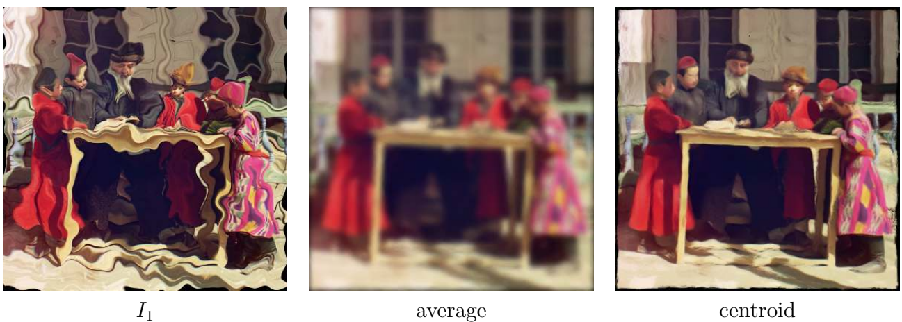
Figure 5: Result of the centroid method over a simulated sequence of 400 frames.
