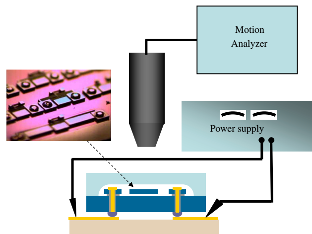
Figure 9. Experimental setup of the MEMS devices driving test; the driving voltage was input from the through-wafer vias.
