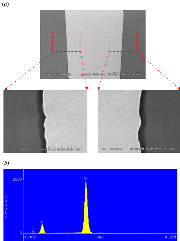
Figure 4. (a) Zoom-in view of the through-wafer vias and a nearby silicon substrate, and (b) the EDX analysis of the insulating material.
