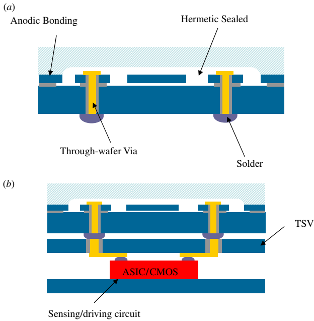
Figure 1. The present packaging model for SOI-MEMS wafer-level hermetic packaging.
