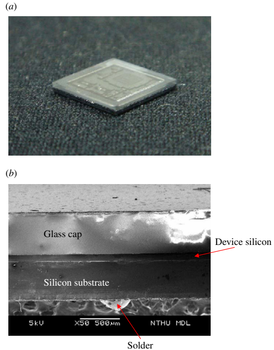
Figure 5. (a) Photo of a packaged SOI-MEMS chip covered by a Pyrex 7740 glass, and (b) the SEM photo of the side view of this packaged chip.
