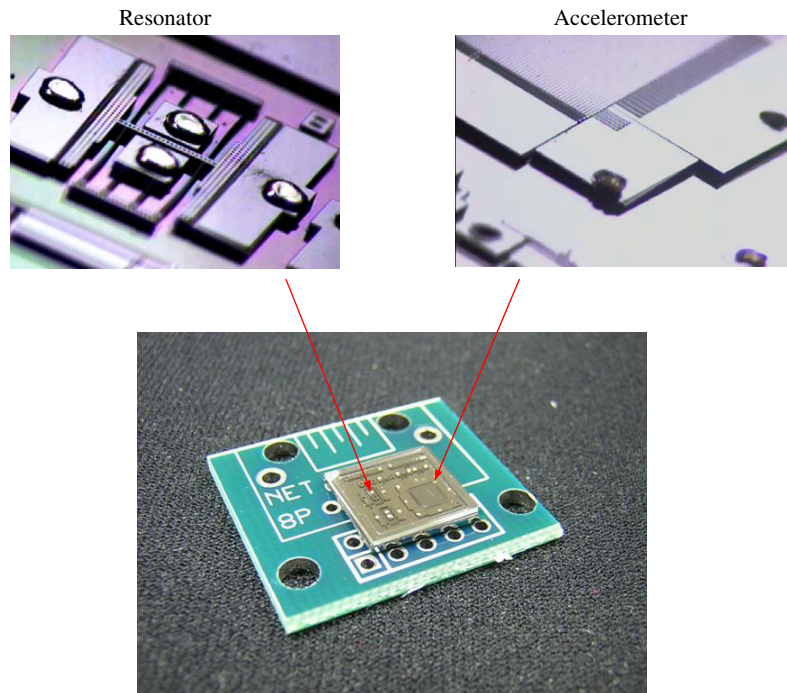
Figure 6. Photo of the packaged SOI-MEMS chip on top of a PCB, and the inset photos are the MEMS devices on the SOI wafer.
