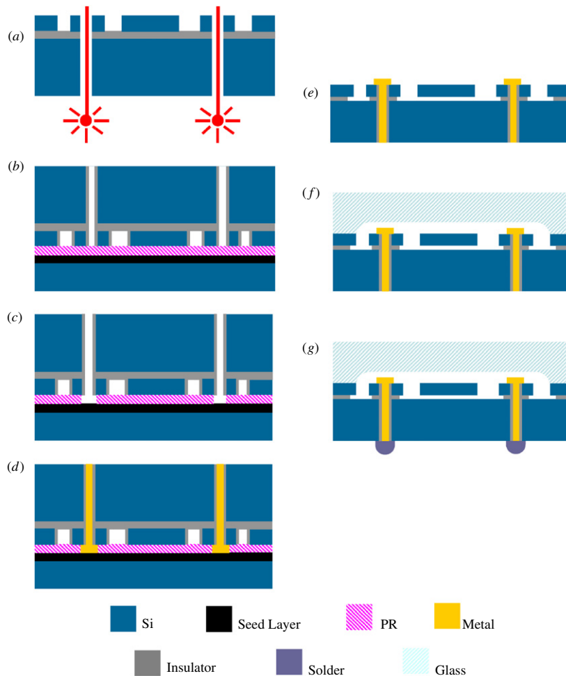
Figure 2. Process flow for SOI-MEMS wafer-level hermetic packaging.
