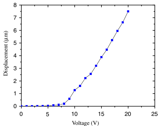
Figure 10. Measured variation of packaged thermal actuator displacements with the driving voltages.
