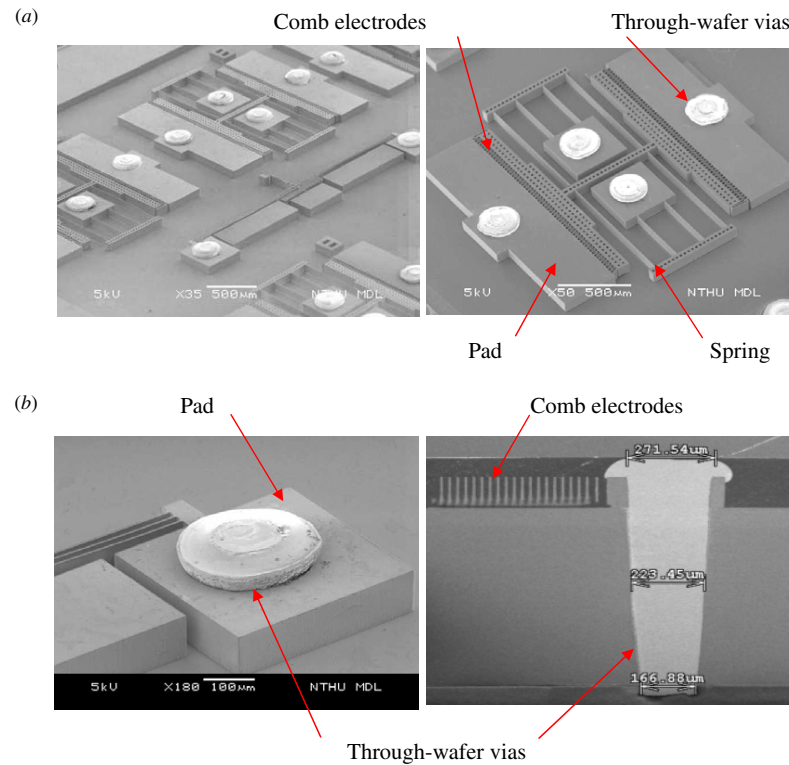
Figure 3. The fabrication results of through-wafer vias and SOI micromachined devices, (a) the SOI micro actuators with bond pads and through-wafer vias and (b) close-up and cross-sectional views of the through-wafer vias.
