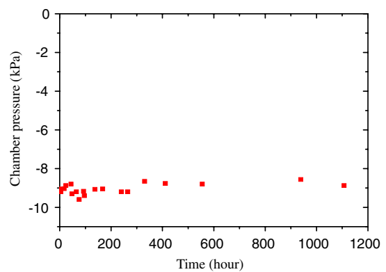
Figure 8. Measured variation of chamber pressure with the time period.
