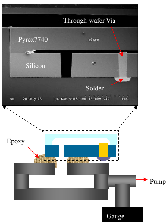
Figure 7. Experimental setup for hermetic testing.
