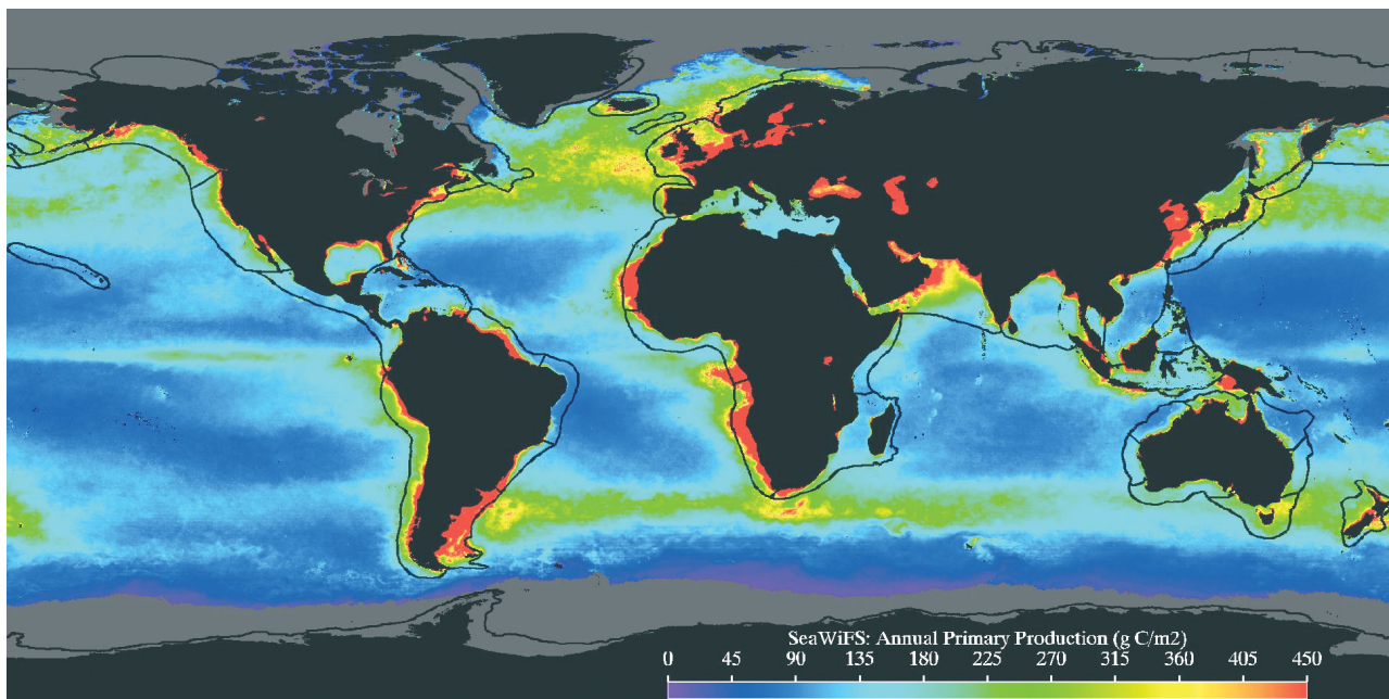
Fig. 4. Boundaries of the 64 Large Marine Ecosystems (LMEs) of the world and primary productivity ( \text{g C m}^{-2} \text{ yr}^{-1} ). Annual productivity estimates are based on SeaWiFS satellite data collected between September 1998 and August 1999, and on the model developed by Behrenfeld & Falkowski (1997). Color-enhanced image provided by Rutgers University (available at: www.edc.uri.edu/lme , Introduction)
