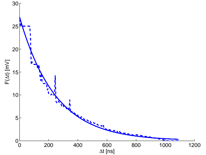
Fig. 6. Measurement of the STDP modification function for a single, arbitrary synapse (dashed line). The theoretical model is shown as a reference (solid line). The parameters were set as follows: A = 27 mV, \Delta t = 245 ns.
