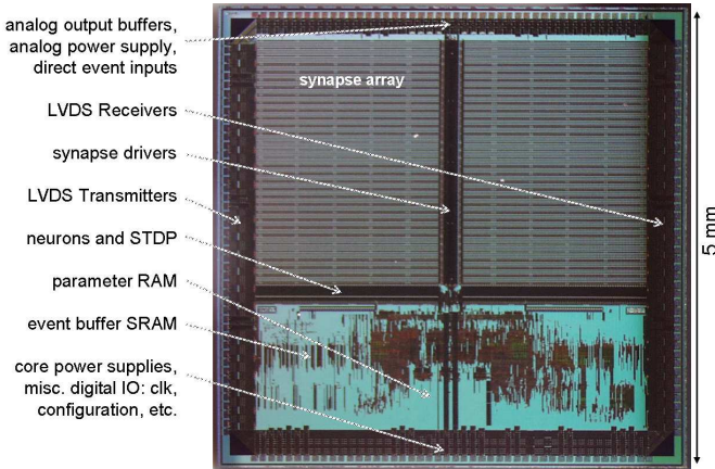
Fig. 3. Die-photograph of the presented neural network chip.
