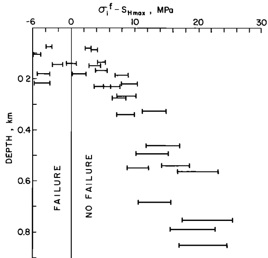
Fig. 5. The difference between the maximum principal stress presumably needed for failure \sigma_1^f and the measured value of this component S_1 as a function of depth; \sigma_1^f (equation (1)) has been calculated for \mu = 0.75 and \mu = 0.85 , and the horizontal bars indicate the range between these two assumptions.
