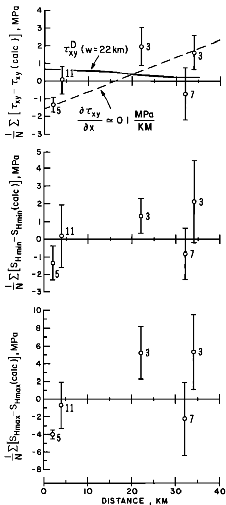
Fig. 6. Average residuals of the stress components as a function of distance from the fault. The calculated stresses are from equations (2), (3), or (4), and the observations are listed in Table 1. The numbers by each point indicate how many measurements were considered in determining a particular residual. In the topmost graph, the stress \tau_{xy}^D due to fault slip of 3.1 m at depths below 22 km is shown as a solid line (equation (11)). The dashed line simply provides an approximate indication of the maximum horizontal gradient in \tau_{xy} that might escape detection due to the localized variation in the observations.
