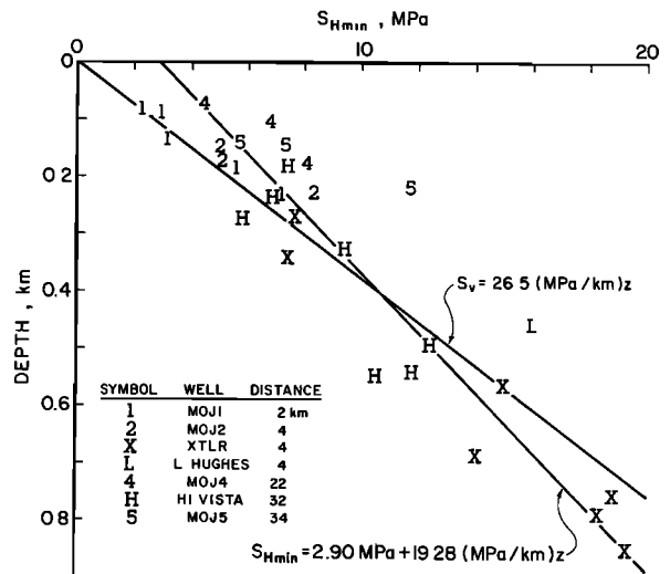
Fig. 3. The minimum horizontal stress S_{Hmin} as a function of depth.
