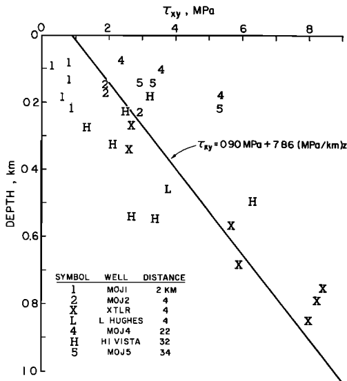
Fig. 2. The horizontal shear stress \tau_{xy} as a function of depth and location.
