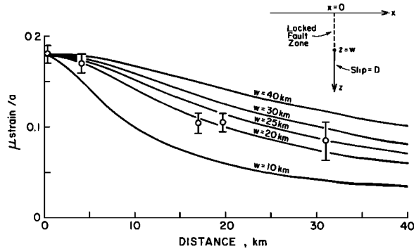
Fig. 7. Rates of strain change \dot{\epsilon}_{xy} averaged over five geodetic networks and theoretical rates of strain change calculated on the basis of the fault zone model schematically illustrated in the upper right hand side of the figure.
