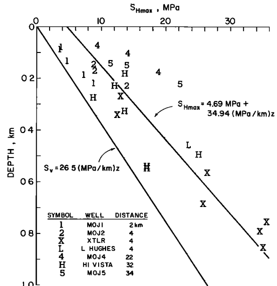
Fig. 4. The maximum horizontal stress S_{Hmax} as a function of depth.
