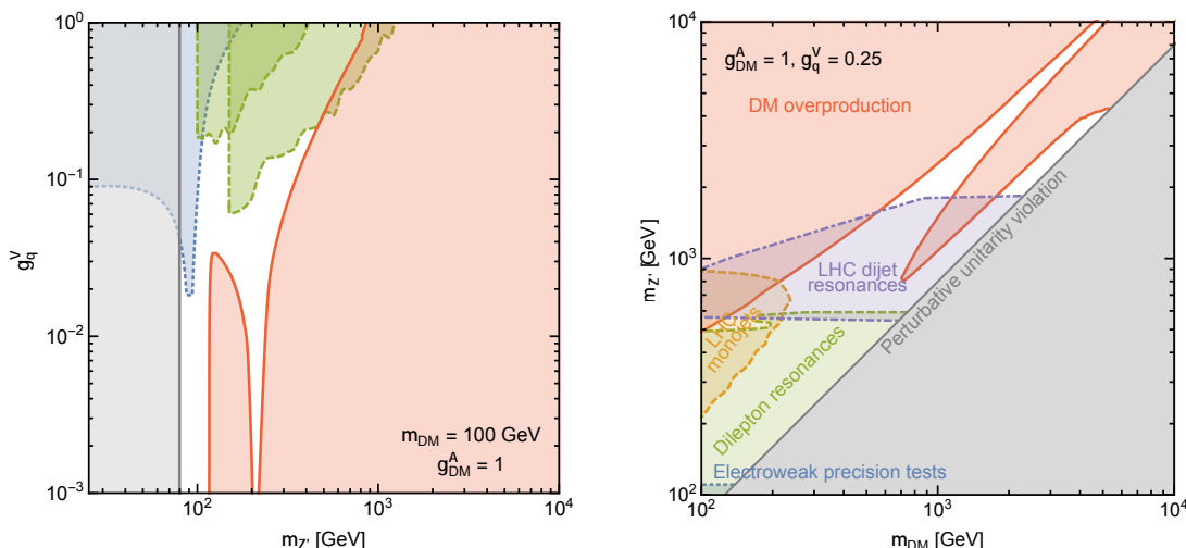
Figure 6. Vector(SM)–Axial(DM): parameter space forbidden by constraints from ATLAS and Tevatron dileptons (green, dashed) and electroweak precision observables (blue, dotted) in the m_{Z'}-g_q^V parameter plane (left) and the m_{DM}-m_{Z'} parameter plane (right), assuming that \epsilon = 0 at \Lambda = 10 TeV so that kinetic mixing is only induced at the one-loop level. In the right panel we show also the region excluded by LHC monojet (orange, dashed) and dijet (violet, dot-dashed) searches due to tree-level Z' exchange for the adopted coupling choice. In both panels we show the parameter space where perturbative unitarity is violated (grey). For the relic density calculation we have assumed that the mass of the hidden sector Higgs saturates the unitarity bound.
