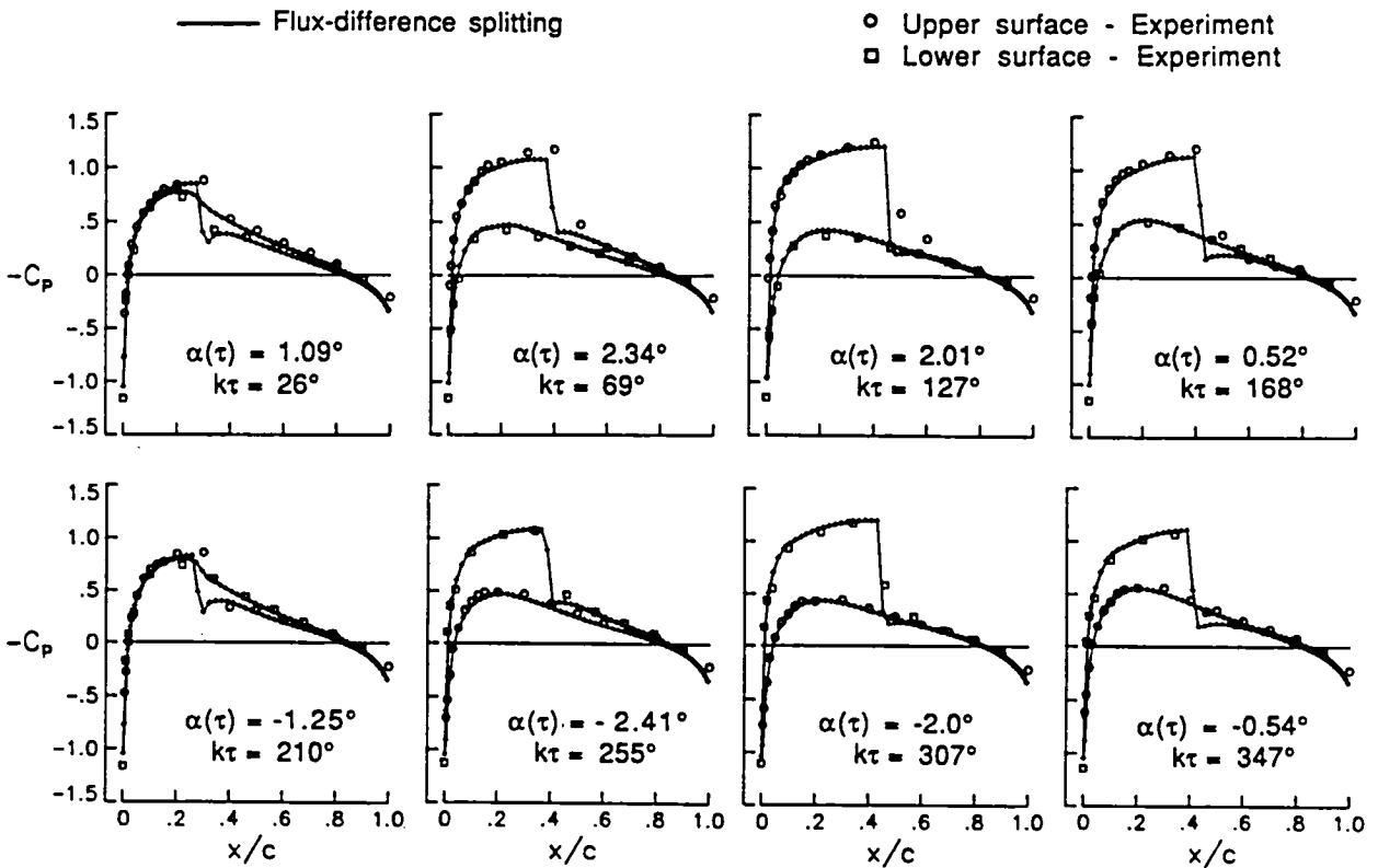
Fig. 8 Comparison of instantaneous pressure distributions for the NACA 0012 airfoil pitching at M_\infty = 0.755 , \alpha_0 = 0.016^\circ , \alpha_1 = 2.51^\circ , and k = 0.0814 computed using flux-difference splitting.
