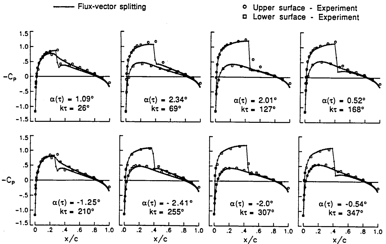
Fig. 7 Comparison of instantaneous pressure distributions for the NACA 0012 airfoil pitching at M_\infty = 0.755 , \alpha_0 = 0.016^\circ , \alpha_1 = 2.51^\circ , and k = 0.0814 computed using flux-vector splitting.
