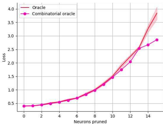
Figure 2: Pruning the first layer of LeNet3 on CIFAR-10 with Combinatorial oracle and Greedy oracle. Networks remain fixed and are not fine-tuned. Results for Greedy oracle are averaged over 30 seeds with mean and standard deviation shown. Best observed results for Combinatorial oracle for every seed are averaged.
