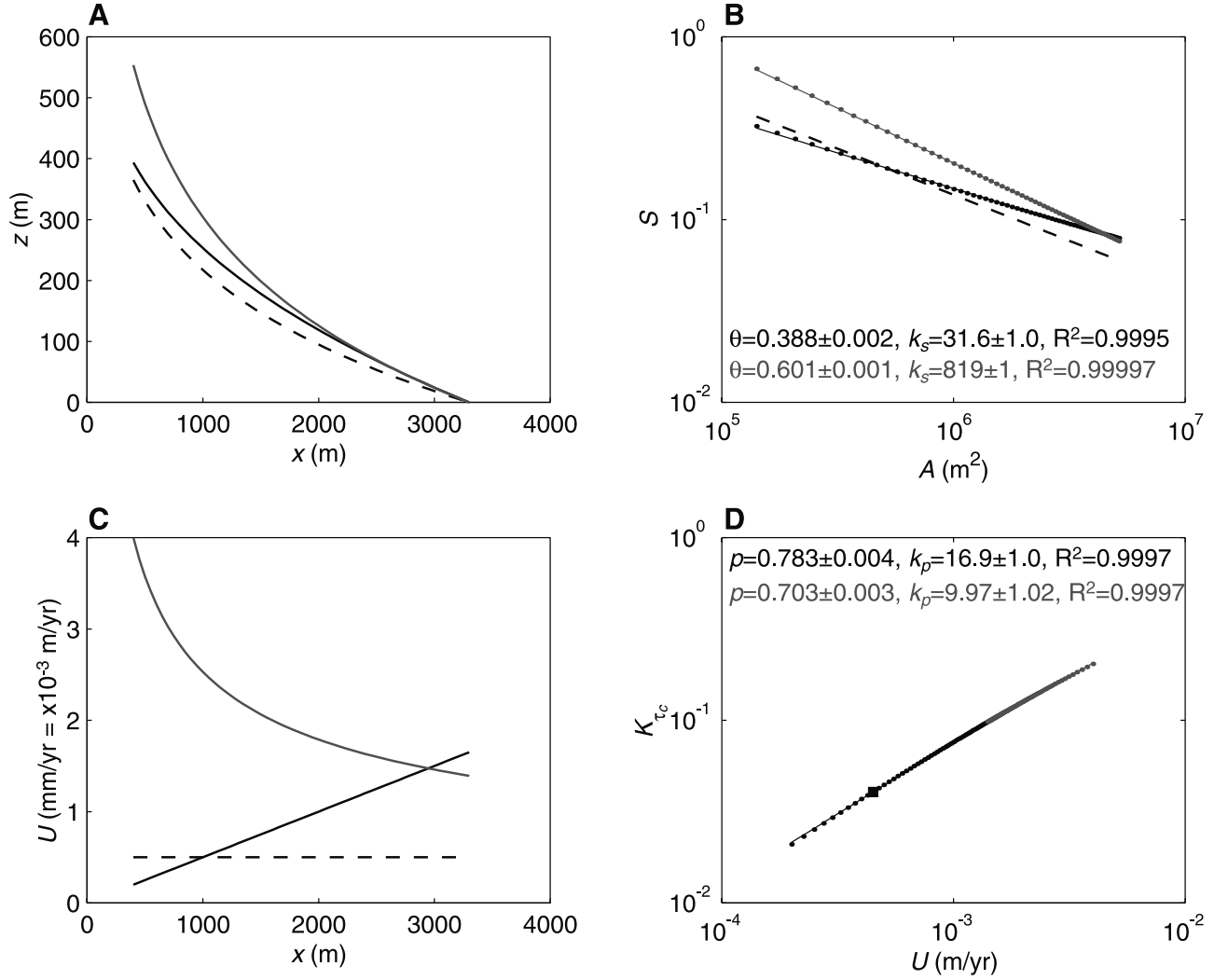
Figure 6. Effect on channel concavity of spatially varying uplift rate ( U ) using the stochastic threshold model. In all frames, the dashed lines show a case with constant U ( U = 0.0005 m yr -1 ), solid lines show a case where U = U(x) . For the black line, U = 5 \times 10^{-7}x , for the gray line, U = 0.08x^{-0.5} . Parameter values for these model runs are the same as those shown on Table 2b for Eureka climate parameters and n = 1 . (a) Steady state channel longitudinal profiles, elevation ( z ) against distance ( x ). Note that the U(x) cases have different concavity. (b) Channel gradient ( S )–drainage area ( A ) power law regressions (equation (6)). The constant U case (dashed line) has \theta = 0.51 = m/n and k_s = 170 . (c) Uplift rate functions used. (d) K_{\tau_c} – U power law regressions, using equation (9a). Box indicates the K_{\tau_c} – U relationship for the constant U case. Note that in the regressions (Figures 6b and 6d) the line (solid) does not perfectly match the data points in the U(x) case due to deviation of the equation (9a) relation from power law form. The difference in the best fit values of p in Figure 6d is solely the result of regression over differing ranges of U . The predicted channel concavity index ( \Theta , equation (11)) for these cases is 0.388 and 0.601, respectively, which matches the observed concavity index ( \theta ) closely.
