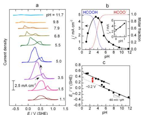
Figure 1. (a) Cyclic voltammograms of a rotating Pt disk electrode (1000 rpm) at 50 \text{ mV s}^{-1} in 0.2 M phosphate buffer solutions or 0.5–1 M H_3PO_4 (for pH < 2 ) containing 50 mM HCOONa. (b) pH dependence of the peak current density ( j_p ) on the negative-going scan. Blue and red dotted traces represent the molar fractions of HCOOH and HCOO^- in the solution. Solid curves are only a guide to the eye. Inset shows j_p examined in 0.1–1 M HClO_4 . Owing to the weaker adsorption of ClO_4^- , j_p is larger than in phosphate solutions. (c) pH dependence of the peak potential, E_p .
