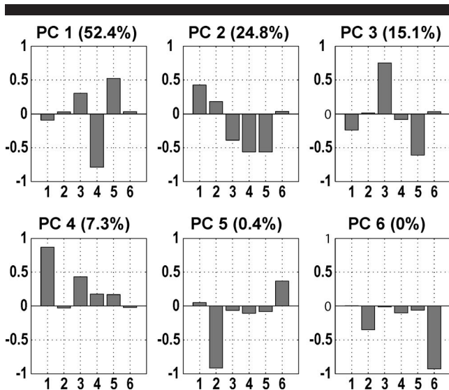
Figure 5. Bar plots of loadings within each principal component (PC) 1–6; percentage of variance explained by each component is shown in parentheses. The variables are 1 = geomorphology; 2 = historical shoreline change rate; 3 = regional coastal slope; 4 = water-level change rate; 5 = mean significant wave height; and 6 = mean tidal range or mean annual ice cover. The percentage corresponds to the amount of variance explained by each PC.
