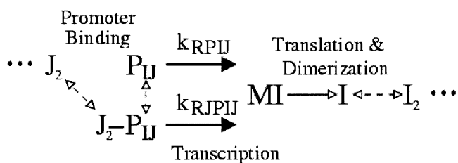
Figure 7 Transcriptional regulatory module. Transcription factor dimer J_2 bind to the promoter, P_{ij} of gene I , influencing the rate of MI transcription. MI is translated into protein I , which dimerizes and then binds to other promoters. Solid arrows indicate irreversible reactions (transcription and translation), dashed arrows indicate reversible promoter binding reactions.
