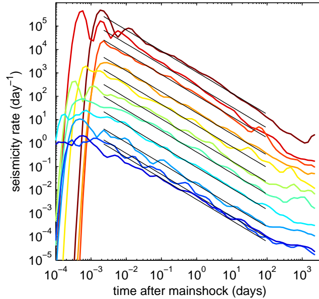
Figure 3. Same as Figure 2 with different parameters D_A = 0.5 \text{ km} , N_{L,A} = 2 , D_F = 3 \text{ km} , N_{L,F} = 3 , and without including aftershocks in the influence zone of previous aftershocks.
