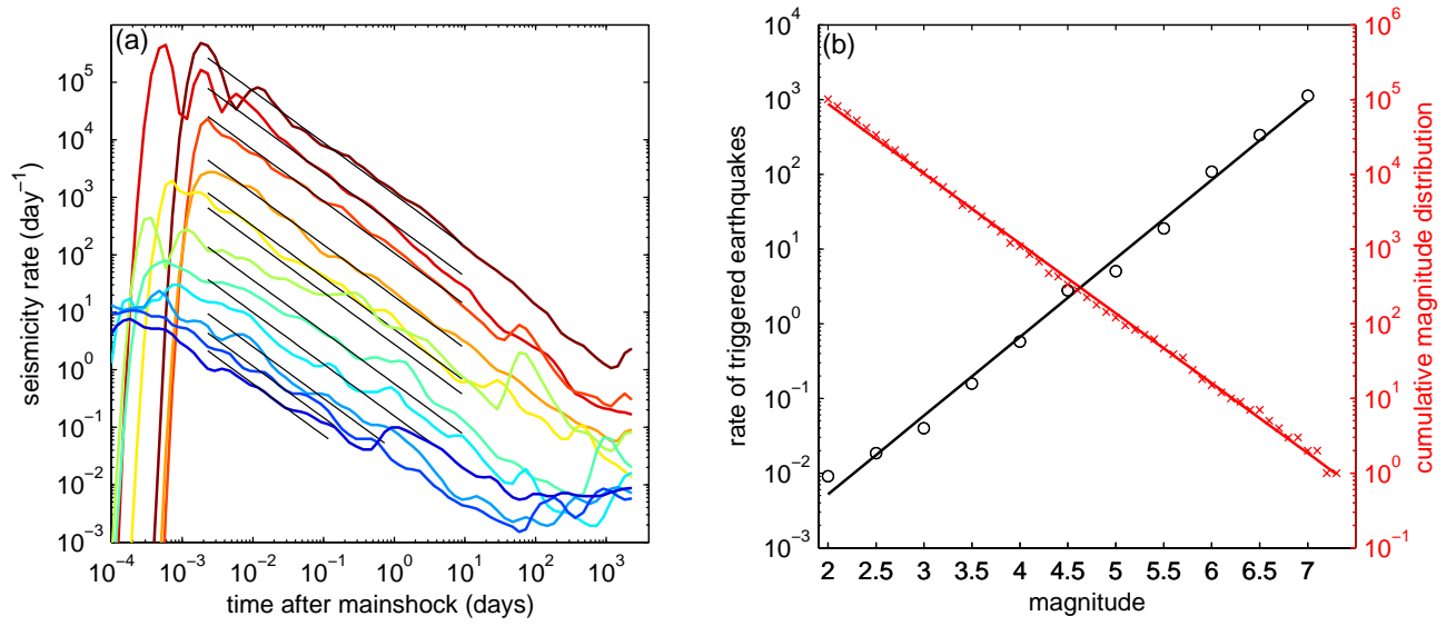
Figure 2. Same as Figure 1 except that we have used m_d = 2 and we have corrected the seismicity rate for missing early aftershocks using (12) (assuming GR law with b = 1 ). We fit the seismicity rate in the time interval 0.002 < t < 10 days and for \lambda(t, m_M) > 0.1 \text{ day}^{-1} . The fit of K(m_M) give K_0 = 0.0041 \text{ day}^{p-1} and \alpha = 1.05 .
