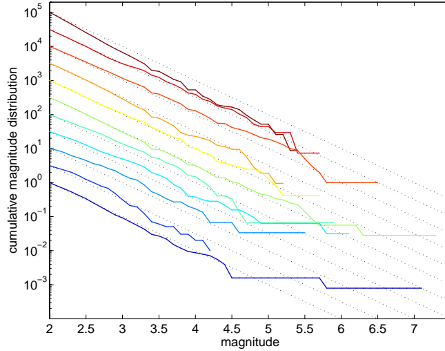
Figure 4. Cumulative magnitude distribution of triggered earthquakes, for mainshock magnitudes ranging from 2 (below) to 7 (top) with a bin size of 0.5. The curves have been normalized by a factor 10^{0.5m_M} for clarity. Dotted lines represent a GR law with b = 1 for reference. The number of events decreases with m_M (between N = 11502 for 7 \leq m_M < 7.5 down to N = 1328 for 7 \leq m_M < 2.5 ) due to the smaller fraction of small earthquakes considered as mainshocks, and due to the shorter time window used for aftershock selection of small mainshocks.
