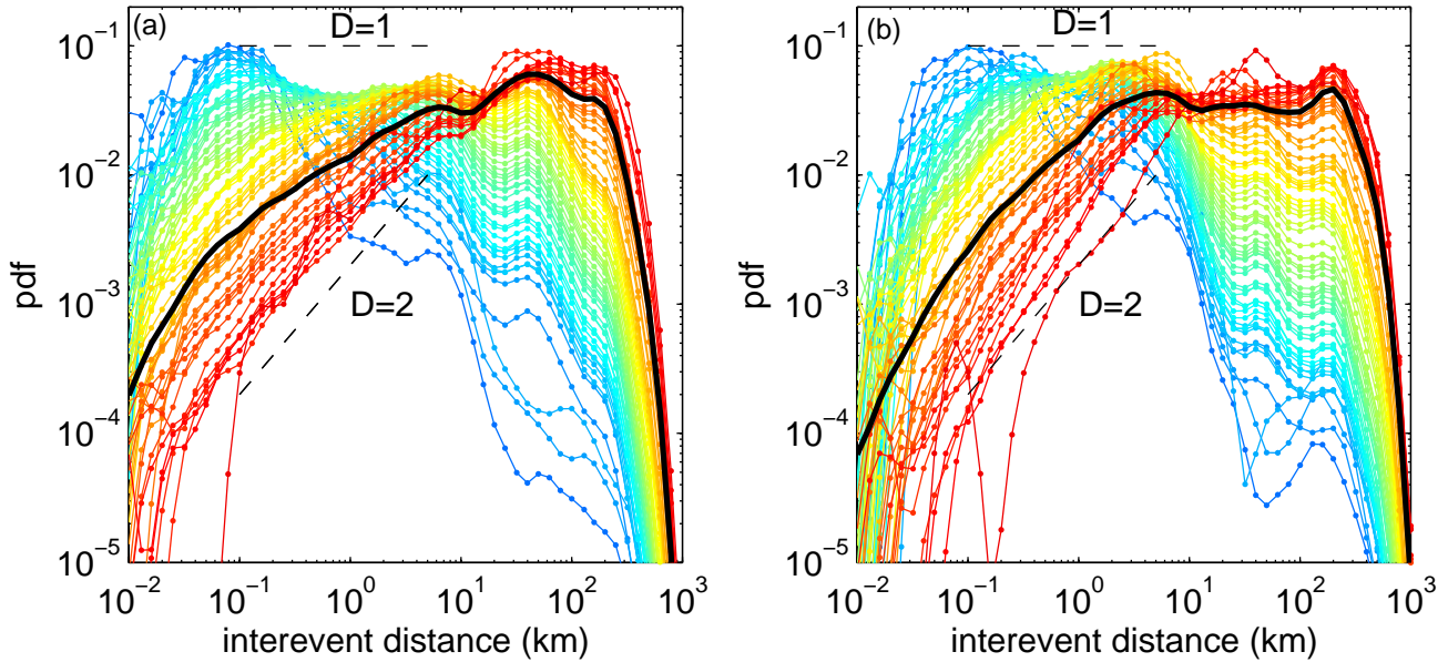
Figure 5. Distribution of distances between hypocenters p_r(r, t) for SHLK (a) and HCS (b) catalogs, using only earthquake pairs with inter-event times in the range [t, 1.25t] , where t increases between 1.4 minutes (blue curve) to 2500 days (red curve). The fractal dimension of p_r(r) , measured for 0.1 \leq r \leq 5 km for all earthquakes (black lines), is D = 1.54 for SHLK catalog and D = 1.73 for HCS catalog.
