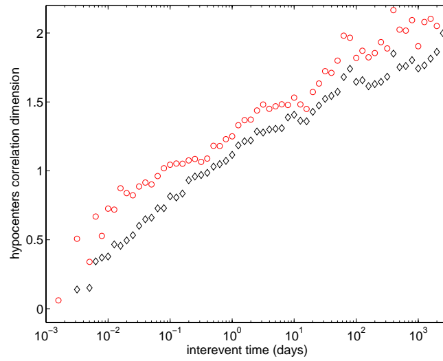
Figure 6. Fractal dimension of p_r(r, t) as a function of inter-event time t , using SHLK catalog (diamonds) and HCS catalog (circles).
