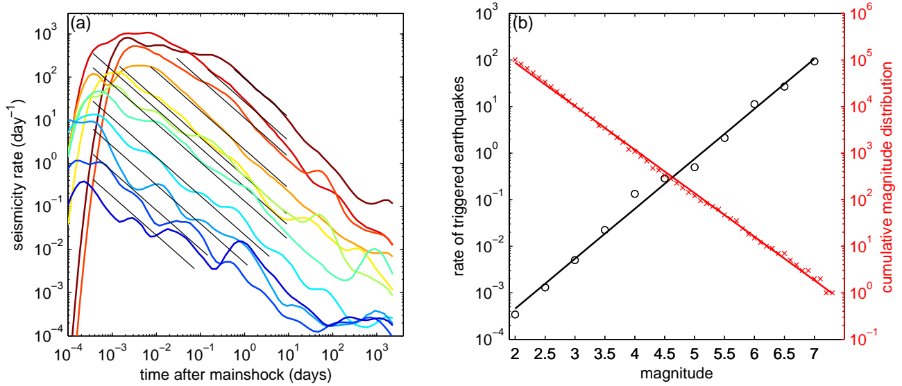
Figure 1. (a) Average rate \lambda(m_M, t) of m \geq 3 earthquakes as a function of the time t after the triggering earthquake, for different values of the magnitude m_M of the triggering earthquake increasing from 2 to 7 with a step of 0.5 from bottom to top. The roll-over at short times is due to the incompleteness of the catalog following a strong mainshock. Black lines show the fit of \lambda(m_M, t) by K(m_M)/t^{0.9} in the time interval [t_{\min}(m_M), t_{\max}(m_M)] , where t_{\min}(m_M) = 0.0003 day (26 sec) for m_M \leq 4.5 mainshocks. For larger mainshocks t_{\min}(m_M) is estimated using expression (12) as the time when the catalog is complete for m \geq 3 . The maximum time is either 10 days or the time when the seismicity rate decays below \lambda_{\min} = 0.01 day -1 . (b) Aftershock productivity K(m_M) as a function of m_M (circles) and cumulative magnitude distribution P(m) (crosses). Solid lines are linear regressions of K(m_M) and P(m) with exponent respectively equal to \alpha = 1.07 and b = 0.94 .
