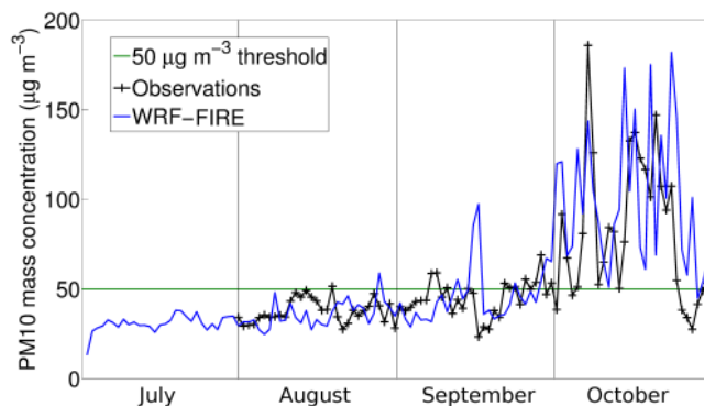
Figure 2. A total of 24h averaged aerosol mass concentration observed (in black crosses) and modeled (in blue line) over Singapore for our study period. The 50 \mu\text{g m}^{-3} indicates the WHO definition of polluted air.
