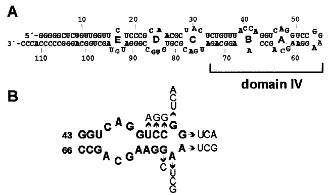
FIGURE 1. 4.5S RNA from E. coli . A: Secondary structure of 4.5S RNA. Internal loops are labeled A–E. B: Base exchanges introduced into the tetraloop region. Single or multiple mutations were introduced as indicated (arrows).
