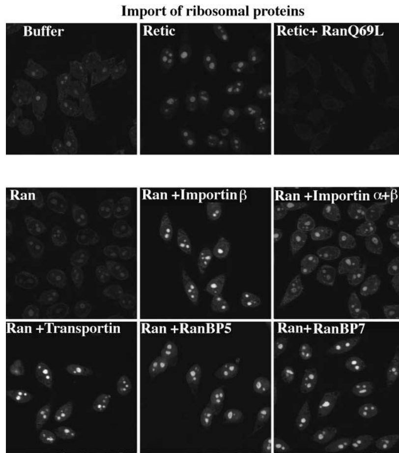
Fig. 1. Nuclear import receptors for ribosomal proteins. Total, fluorescein-labelled ribosomal proteins were prepared from canine ribosomes as described in Materials and methods and used as the substrate for import into nuclei of permeabilized HeLa cells. Import was for 15 min at room temperature in the presence of an energy-regenerating system. Where indicated, the import reaction contained the following additions: reticulocyte lysate (Retic); 3 \mu M RanQ69L; a Ran-mix (Ran) containing 4 \mu M RanGDP, 0.4 \mu M RanBP1, 0.4 \mu M Schizosaccharomyces pombe Rna1p and 0.4 \mu M NTF2 (each final concentrations); 2 \mu M importin \beta ; 2 \mu M importin \beta + 6 \mu M importin \alpha ; 3 \mu M transportin; 3 \mu M RanBP5; or 3 \mu M RanBP7. The reactions were stopped by fixation and import was analysed by confocal fluorescence microscopy. Note that efficient nucleolar accumulation of the ribosomal proteins occurred in the presence of either reticulocyte lysate, importin \beta , transportin, RanBP5 or RanBP7. The RanQ69L mutant had a strong dominant-negative effect.
