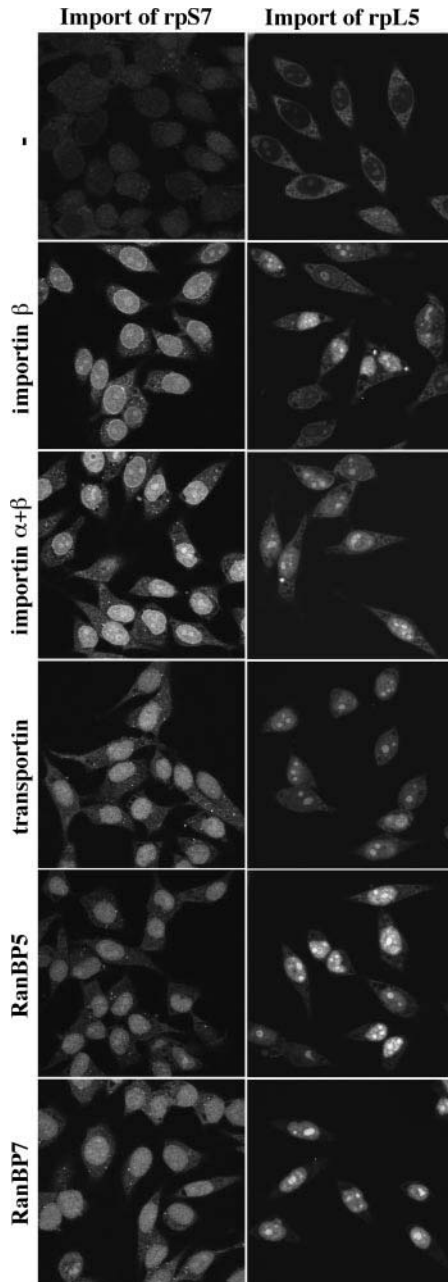
Fig. 5. Nuclear import of ribosomal proteins S7 and L5. Import in the presence of energy and Ran was performed and analysed as in Figure 4, using fluorescent fusions with rpS7 and rpL5 as substrates.
