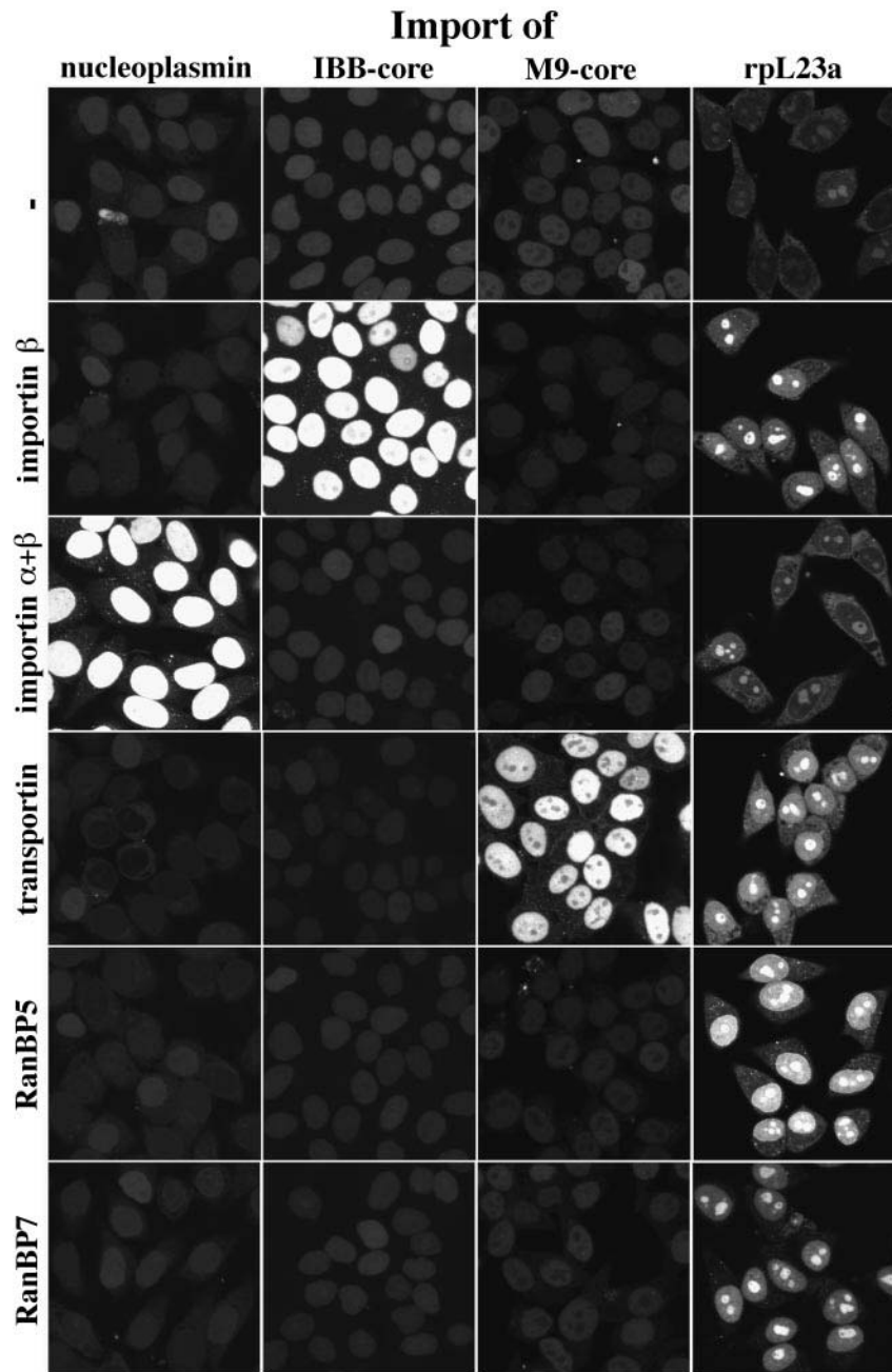
Fig. 4. rpL23a can be imported into the nucleus via four distinct pathways. Nuclear import of the indicated fluorescein-labelled import substrates ( \approx 4 \mu\text{M} each) was performed in the presence of a Ran mix (see Figure 1), an energy-regenerating system and either buffer, 1.5 \mu\text{M} importin \beta , 1.5 \mu\text{M} importin \beta + 4.5 \mu\text{M} importin \alpha , 4 \mu\text{M} transportin, 4 \mu\text{M} RanBP5 or 2.5 \mu\text{M} RanBP7. Reactions were stopped after 15 min by fixation, and import was analysed by confocal fluorescence microscopy. Note that efficient import of nucleoplasmin was only observed with importin \alpha + \beta , that of the IBB fusion only with importin \beta , and that of the M9 fusion only with transportin. In contrast, import of the ribosomal protein L23a was efficient either with importin \beta , transportin, RanBP5 or with RanBP7.
