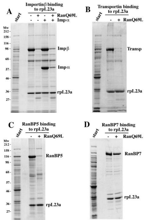
Fig. 3. Direct interaction of rpL23a with nuclear transport receptors. Immobilized rpL23a was used to bind either (A) recombinant importin \beta , (B) transportin, (C) RanBP5 or (D) RanBP7 out of total E. coli lysates. Where indicated, 10 \mu M RanQ69L GTP or 5 \mu M Xenopus importin \alpha had also been added. Analysis of the starting material and bound fraction was by SDS-PAGE followed by Coomassie staining. The load in the bound fractions corresponds to 15 times the starting material. Note that importin \beta , the importin \alpha/\beta heterodimer, transportin, RanBP5 and RanBP7 all bound specifically to rpL23a. RanQ69L strongly reduced binding of all these factors, except for RanBP7 where the effect was weaker. It should also be noted that the (minor) background bands in the bound fractions in (A) and (C) are mainly proteolysis products from importin \beta (A) or RanBP5 (C).
