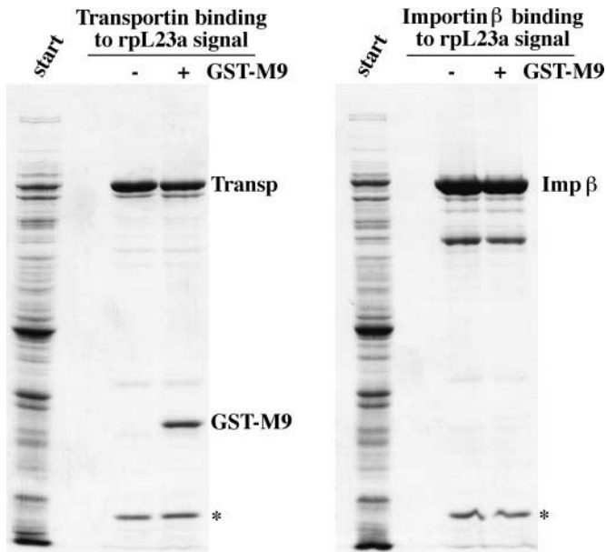
Fig. 7. Transportin has distinct binding sites for the M9 domain and the L23a interaction domain. Binding of transportin or importin \beta to residues 32–74 of rpL23a (BIB domain) was performed as described in Figure 4. Note that the addition of 5 \mu M of the GST–M9 fusion did not compete the rpL23a–transportin interaction. Instead, GST–M9 was recovered in the bound fraction, indicating the formation of a trimeric L23a–transportin–M9 complex. As a control, GST–M9 was not bound if transportin was replaced by importin \beta (right panel). The asterisk denotes 2z–BIB fusion protein that had leaked from the column.
