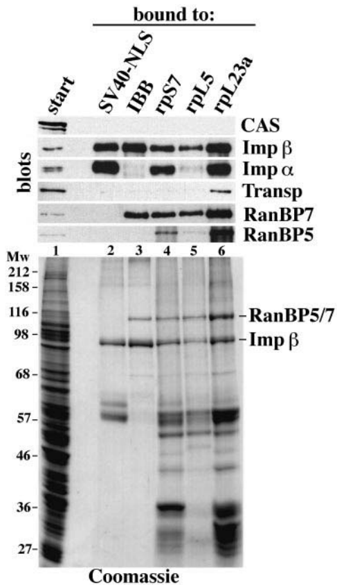
Fig. 2. Ribosomal proteins interact with multiple cytosolic transport receptors. The ribosomal proteins S7, L5 and L23a were immobilized and tested for binding of nuclear transport receptors from a Xenopus egg extract. Positive controls were binding to an immobilized SV40 NLS peptide-BSA conjugate (specific for the importin \alpha/\beta heterodimer) or to the IBB domain from importin \alpha (specific for importin \beta and the importin \beta -RanBP7 heterodimer). Each 20 \mu l of the resins was incubated with 500 \mu l of egg extract (HSS). After extensive washing, bound proteins were eluted with 1.5 M MgCl_2 , precipitated and analysed by SDS-PAGE followed by immunoblotting with specific antibodies or by Coomassie staining. The load in the bound fractions corresponds to 25 times the starting material. The positions of RanBP5, RanBP7 and importin \beta in the Coomassie gel are indicated. Transportin would co-migrate with importin \beta .
