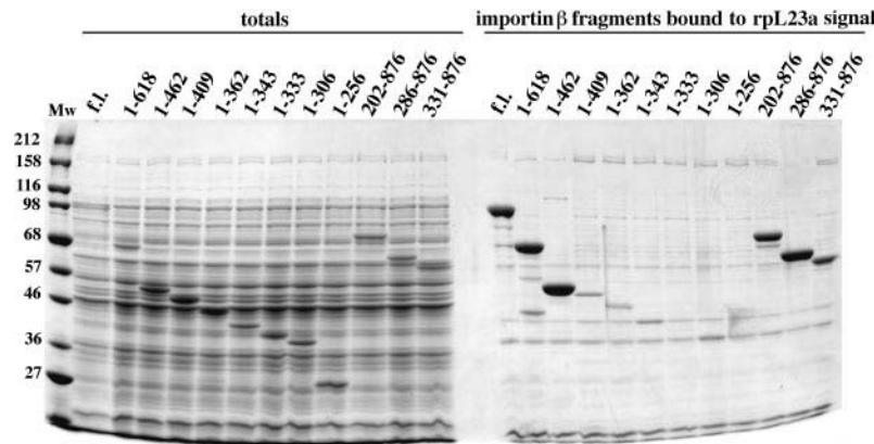
Fig. 8. Definition of a binding domain in importin \beta for rpL23a. The importin \beta fragments, as indicated above the lanes, were tested for binding to the immobilized BIB domain from rpL23a (residues 32–74). f.l. stands for full-length importin \beta , i.e. residues 1–876. Starting materials and bound fractions were analysed by SDS–PAGE and Coomassie staining. The load in the bound fractions corresponds to 10 times the starting material. Note that residues 286–462 of importin \beta are essential for high-affinity interaction with the rpL23a import signal.
