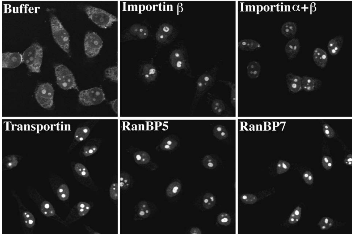
Fig. 6. Residues 32–74 of rpL23a constitute a universal NLS that accesses multiple import pathways. Import was performed and analysed essentially as in Figure 4, using a fluorescent fusion with residues 32–74 from rpL23a (i.e. the BIB domain) as a substrate.
