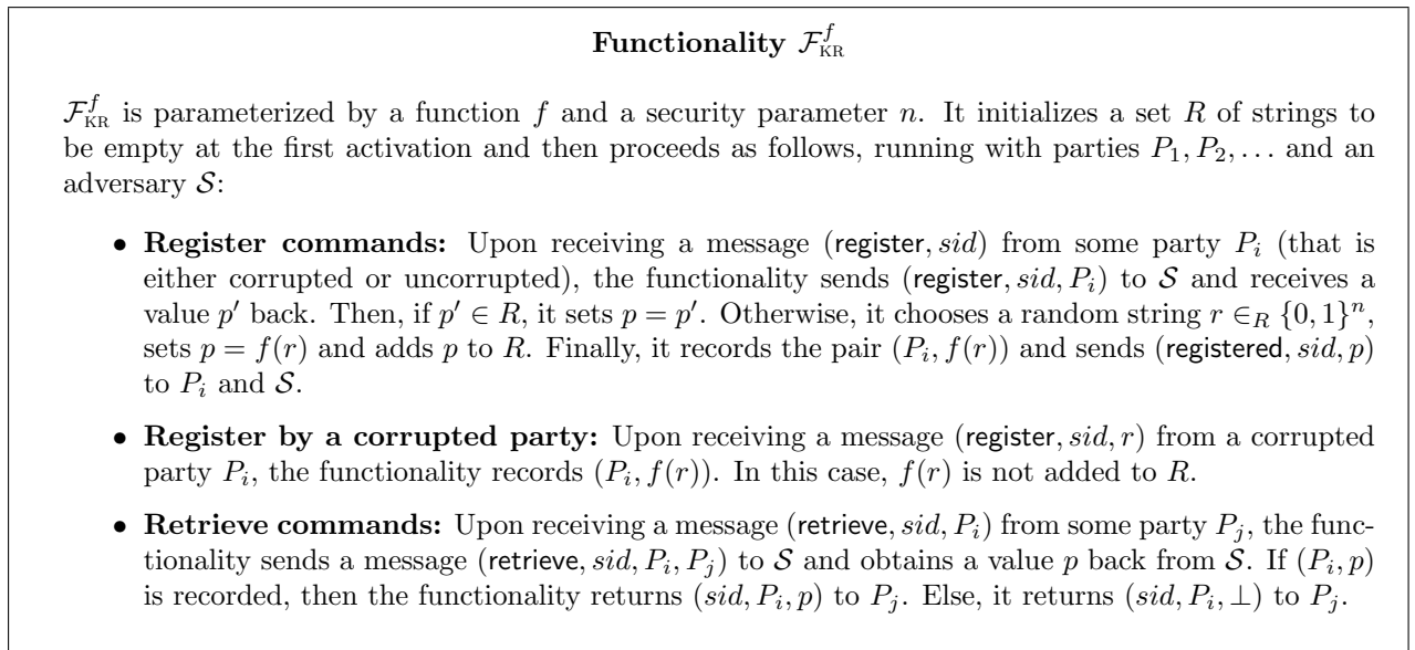
Figure 5: The key registration functionality of [2]
