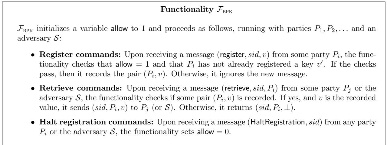
Figure 4: The bare public-key model functionality
