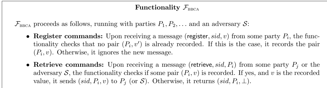
Figure 1: The Bulletin-Board CA functionality
