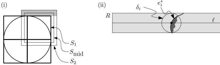
Fig. 4 Illustration for the proof of Lemma 3.1
