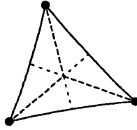
Fig. 3. Barycentric subdivision.
