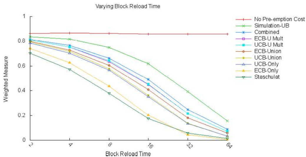
Fig. 14 Weighted schedulability measure; varying block reload time from 2^0 = 1 \mu\text{s} to 2^4 = 32 \mu\text{s}
