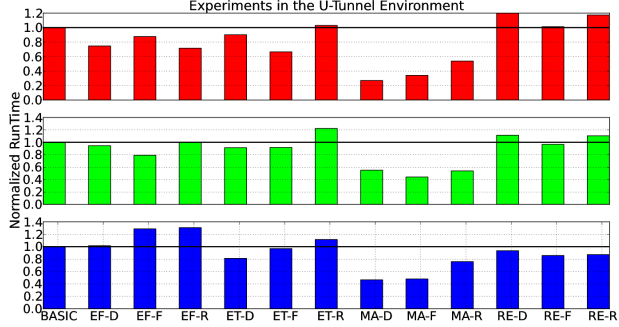
Fig. IV.8. Total C_{free} mapping time normalized over the corresponding “Basic” sampling-based method in our 6DOF U-Tunnel environment.
