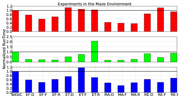
Fig. IV.7. Total C_{free} mapping time normalized over the corresponding “Basic” sampling-based method in our 2DOF Maze environment.
