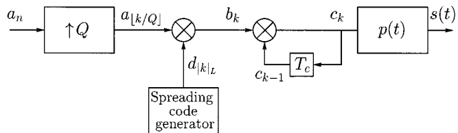
Fig. 1. Modulator block diagram.
