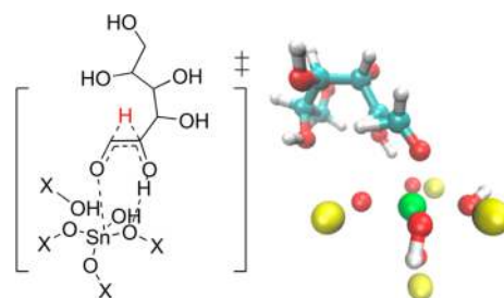
Figure 10. Rate-limiting transition state for glucose–fructose isomerization catalyzed by Sn-BEA.
