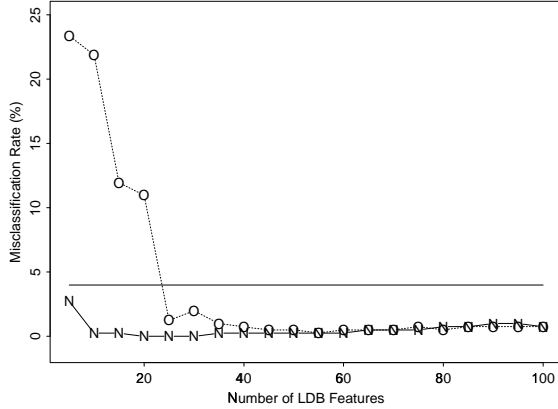
Figure 1: Misclassification rates using LDA as a classifier versus the number of the top LDB features retained. The plots with symbols O and N correspond to the results using the original and the new LDB algorithms, respectively. The constant level line about 4% indicates the performance of the LDA directly applied to the signals represented in the standard coordinate system (of 256 time samples).
