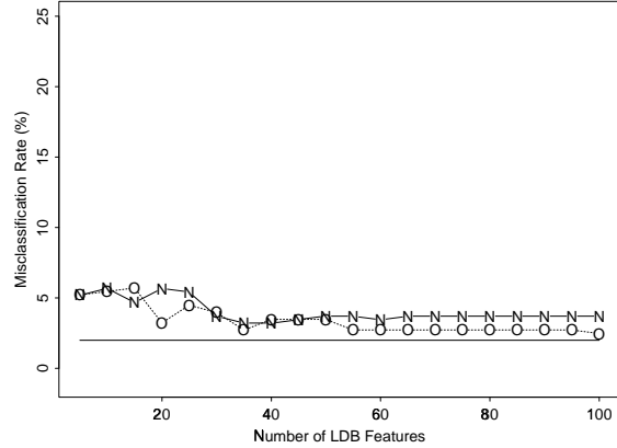
Figure 2: Misclassification rates using CT as a classifier versus the number of the top LDB features retained. The constant level line about 2% indicates the performance of the CT directly applied to the signals represented in the standard coordinate system.
