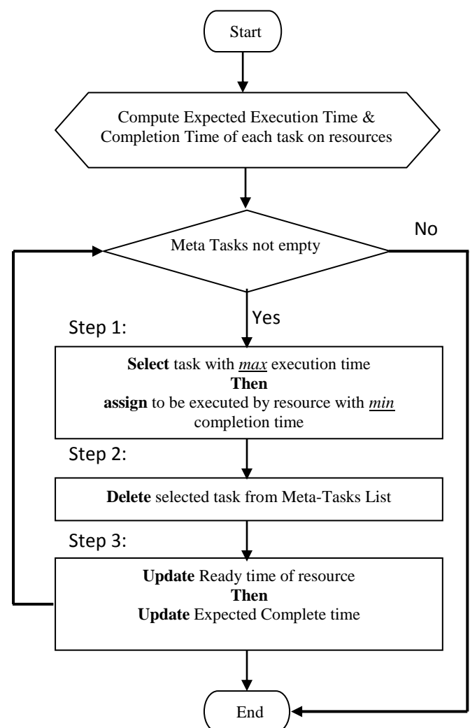
Fig 3: Improved Max-Min Flowchart
