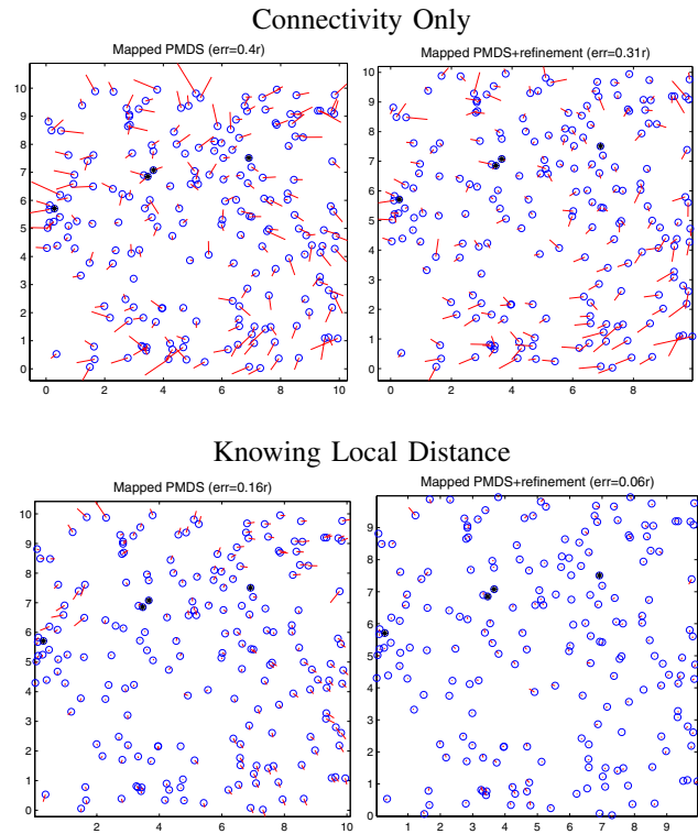
Fig. 7. Results of MDS-MAP(P) and MDS-MAP(P,R) on the example of random uniform placement. The upper two diagrams show their results using connectivity information only, whereas the lower two diagrams show their results using distance measures between neighboring nodes with 5% distance errors.
