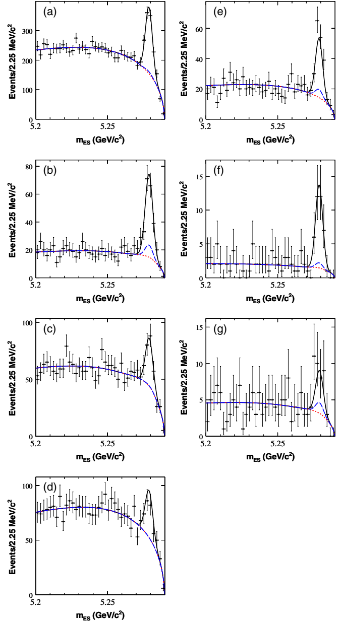
FIG. 2 (color online). Distributions of m_{ES} in \Delta E signal region for (a), (e) B^- \rightarrow \tilde{D}^0 K^- , (b), (f) B^- \rightarrow \tilde{D}^{*0}[\tilde{D}^0 \pi^0]K^- , (c), (g) B^- \rightarrow \tilde{D}^{*0}[\tilde{D}^0 \gamma]K^- , and (d) B^- \rightarrow \tilde{D}^0 K^{*-} , with (a)–(d) \tilde{D}^0 \rightarrow K_S^0 \pi^+ \pi^- and (e)–(g) \tilde{D}^0 \rightarrow K_S^0 K^+ K^- . The curves superimposed represent the projections of the fit described in Sec. II C: signal plus background (solid black lines), the continuum plus B\bar{B} background contributions (dotted red lines), and the sum of the continuum, B\bar{B} , and K/\pi misidentification background components (dashed blue lines).
