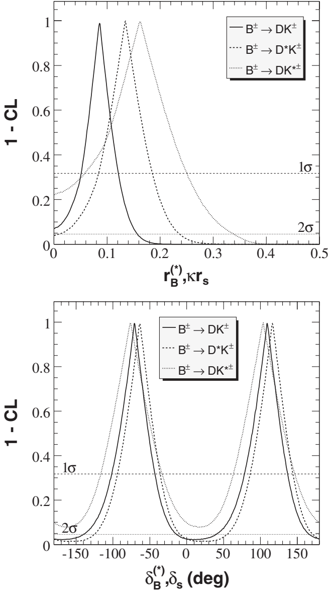
FIG. 13. \alpha = 1 - \text{CL} as a function of (upper panel) r_B, r_B^* , and \kappa r_s , and (lower panel) \delta_B, \delta_B^* , and \delta_s , for B^- \rightarrow \tilde{D}^0 K^- , B^- \rightarrow \tilde{D}^{*0} K^- , and B^- \rightarrow \tilde{D}^0 K^{*-} decays, including statistical and systematic uncertainties and their correlations. The dashed (upper) and dotted (lower) horizontal lines correspond to the 1- and 2-standard-deviation intervals, respectively.
