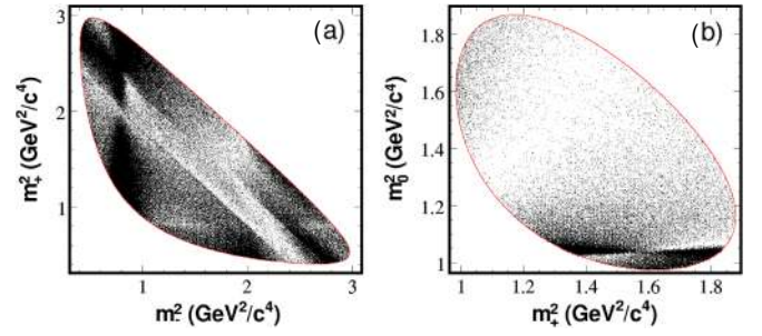
FIG. 5 (color online). Dalitz plot distributions for (a) D^0 \rightarrow K_S^0 \pi^+ \pi^- and (b) D^0 \rightarrow K_S^0 K^+ K^- from D^{*+} \rightarrow D^0 \pi^+ events after all selection criteria, in the D^0 mass signal region. The contours (solid red lines) represent the kinematical limits of the D^0 \rightarrow K_S^0 \pi^+ \pi^- and D^0 \rightarrow K_S^0 K^+ K^- decays.
