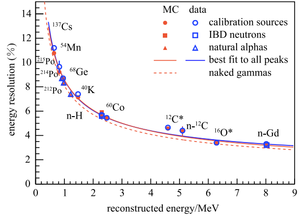
Fig. 20. (color online) Energy resolution for a variety of calibration sources as well as the IBD neutron capture gamma peaks for both MC and data. The parameters in the energy resolution function were extracted by fitting the calibration energy peaks and widths. Alpha source data were used to cross-check the result. The naked gamma sources are also simulated.
