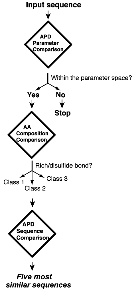
Fig. 3 Prediction of antimicrobial peptides based on the antimicrobial peptide database. The prediction consists of three steps. As the first step, the program will determine whether the input sequence is in the database-defined parameter space (such as charge and hydrophobic content). If identical, the users will be informed. If one or more calculated parameters of the input peptide are out of the boundaries, it is predicted as “your sequence is less likely to be an antibacterial peptide.” Second, the input sequence will be classified into three families: rich in amino acids such as histatins and tryptophans, disulfide-linked peptides, and linear. Third, sequence alignments will be conducted to find five peptides that are most similar to the query sequence
