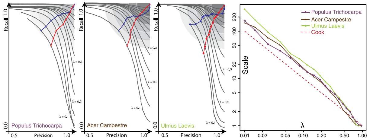
Figure 7: The first three graphs show PR-values for three different tree models. The blue graph shows the optimal scaling values s_{opt} , the red one the standard scaling values s_{Cook} (according to Cook et al. ). For rendering we choose \lambda such that we maintain a minimum quality that is required for a given viewing distance. The minimum quality requirements are indicated by the circles centred at the top-right corner of the PR diagram. As we can see, it is possible to reduce the geometry to a larger extend for model Populus Trichocarpa compared to model Acer Campestre, in particular for small values of \lambda . Right: a log-log plot of scale versus fraction of remaining geometry, that is \lambda . Note that the connected (s_{opt}, \lambda) and (s_{Cook}, \lambda) lines in the PR diagram (left three plots) look very rough. The values plotted against the geometry level \lambda , however, are smooth with the expected exponential behavior. The smoothness is important to avoid popping artefacts during rendering. The \lambda -values are sampled with 0.05 step size from \lambda = 0.1 to 0.4 and with step size 0.1 above.
