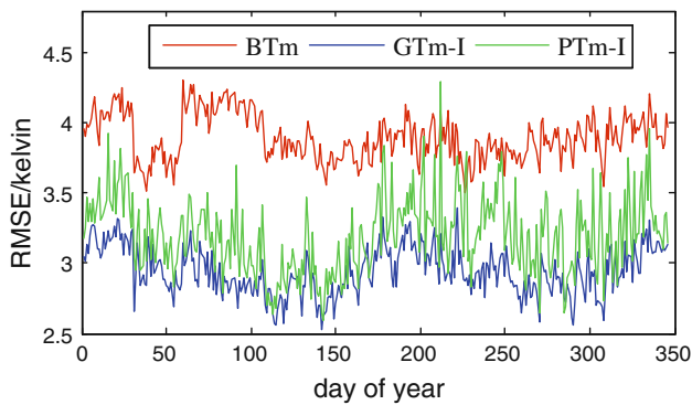
Fig. 6 Daily RMSE of the three models in the early 346 days of 2010 compared with COSMIC-derived T_m data
