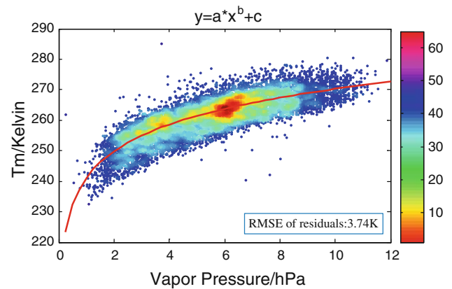
Fig. 2 Plots of the T_m versus e_s and fitting curves of four fitting equations (color indicates data density)
