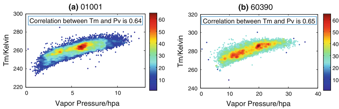
Fig. 1 Plots of T_m versus e_s from 1995 to 2011 at radioonde stations 01001 and 60390 (color indicates data density)
