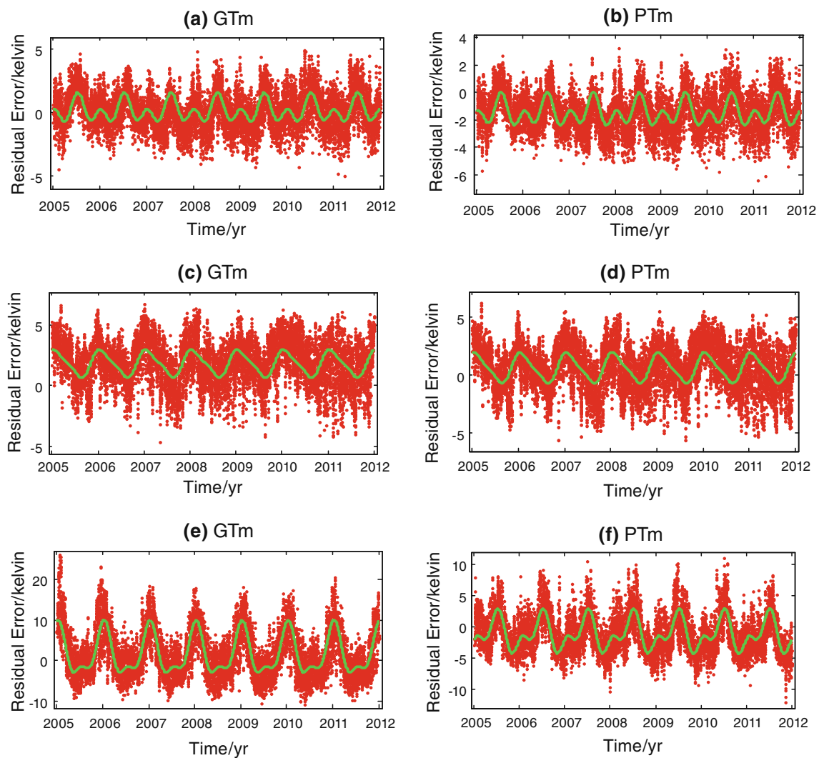
Fig. 4 Residuals (true values – model values) of the GTm model and the PTm model from 2005 to 2011 at N0^{\circ}E7.5^{\circ} , N20^{\circ}E180^{\circ} and N60^{\circ}E160^{\circ} with respect to GGOS atmosphere data
