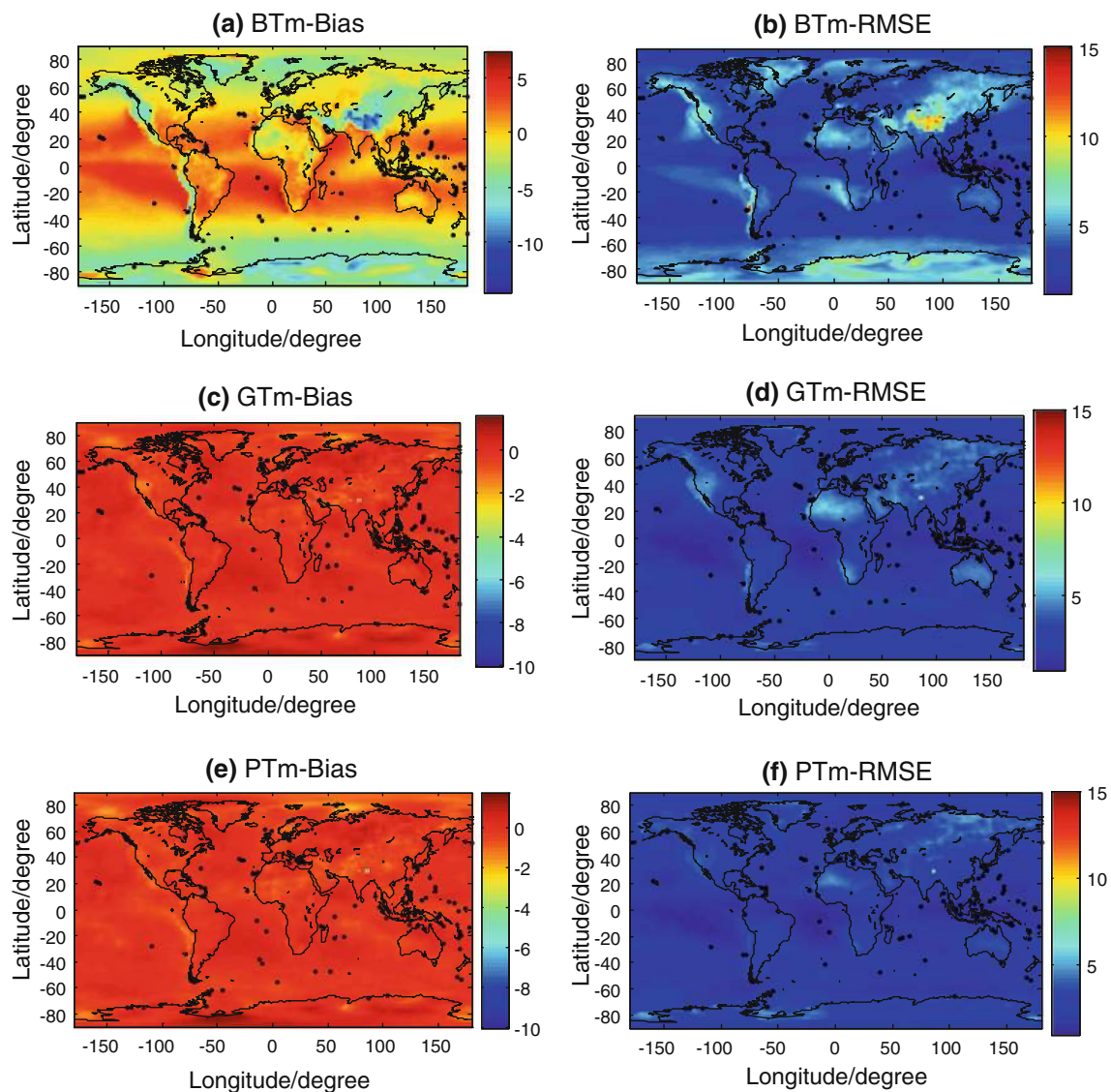
Fig. 5 Global distribution of mean bias and mean RMSE between “GGOS Atmosphere” data and the four models in 2012
