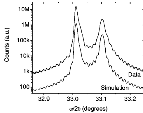
FIG. 2. (004) \omega/2\theta HRXRD spectrum of the \text{GaN}_{0.0063}\text{As}_{0.9937} sample with its corresponding simulated spectrum.
