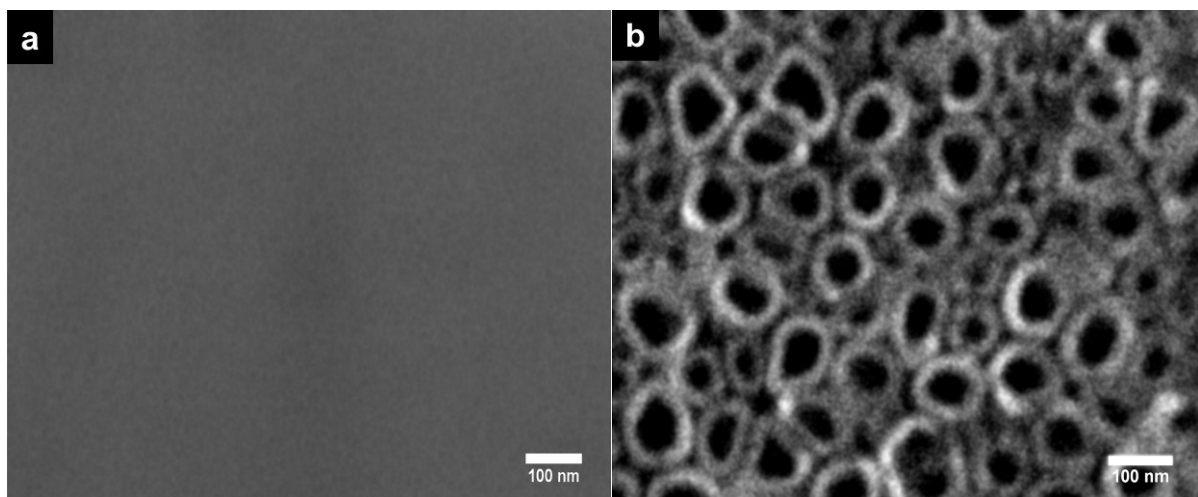
Figure 1. SEM micrographs of the experimental Ti6Al4V alloys. (a) Non-anodized flat Ti6Al4V alloy; (b) anodized Ti6Al4V alloy with NTs.
