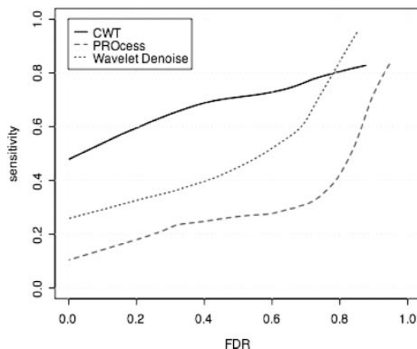
Fig. 6. Comparison of algorithm performance based on FDR-sensitivity relationship.
