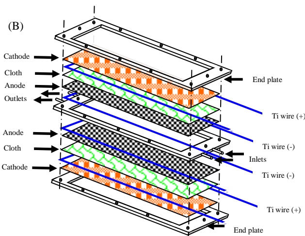
Fig. 1 (A) A photo of the experimental setup testing the large MFC. 1. Feed bottle, 2. Feed pump, 3. Recirculation pump (optional), 4. Recirculation bottle, 5. Larger reactor, 6. Tilt angle adjusting device for the reactor, 7. Outlets level control device, 8. Effluent reservoir, 9. Precision resistor box, 10. Gas sampling port, 11. Effluent outlet. (B) Schematic of the large reactor with double cloth-electrode-assemblies.
