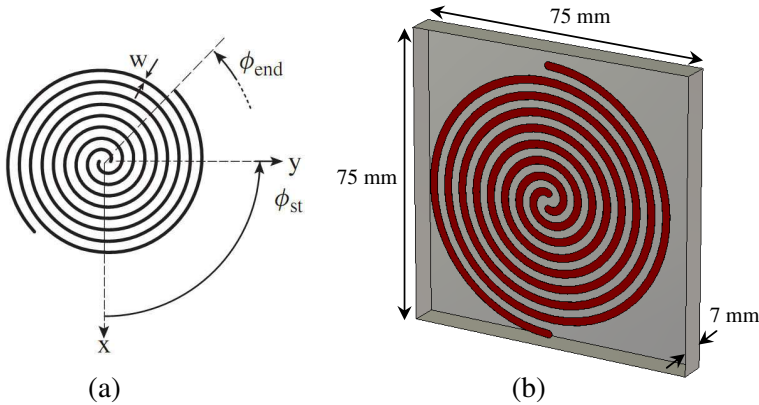
Figure 1. (a) Dimensions of the ARSPL antenna. (b) Configuration of the designed cavity backed ARSPL antenna.
