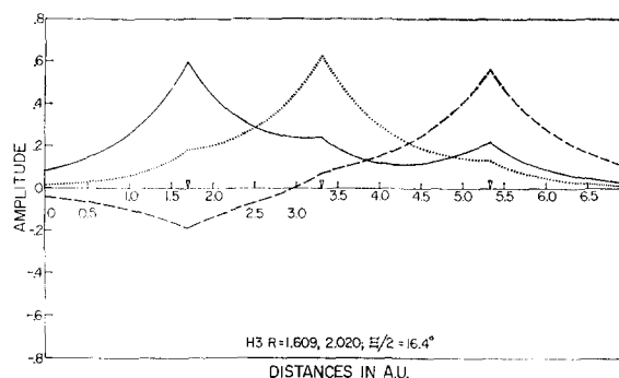
FIG. 5. SOGI orbitals for H_3 : R_{AB}=1.609 , R_{BC}=2.020 ; \Xi/2=16.4^\circ . — orbital 1, \cdots orbital 2, --- orbital 3.
