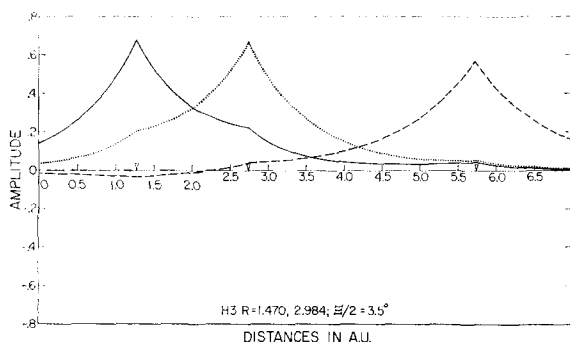
FIG. 4. SOGI orbitals for H_3 : R_{AB}=1.470 , R_{BC}=2.984 ; \Xi/2=3.5^\circ . — orbital 1, \cdots orbital 2, --- orbital 3.
