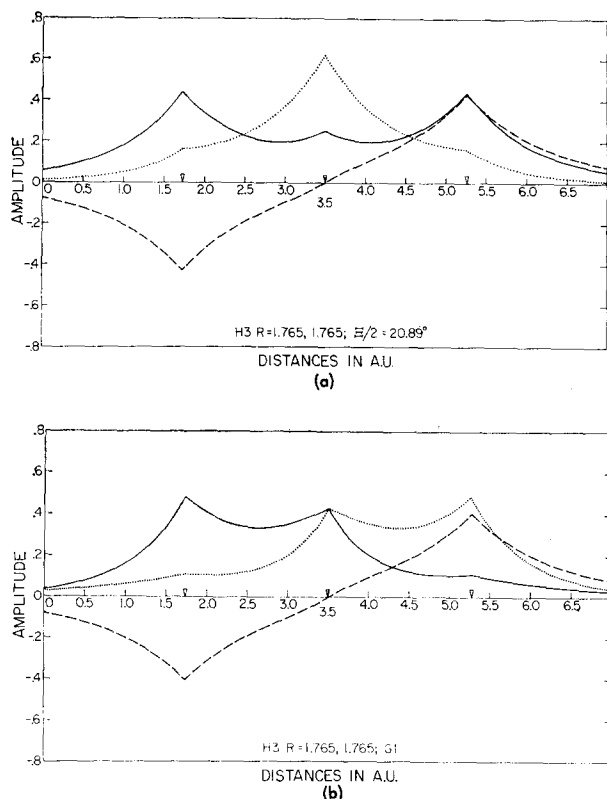
FIG. 6. (a) SOGI orbitals for the saddle point of H_3 : R_{AB} = R_{BC} = 1.765 , E/2 = 20.89^\circ . — orbital 1, ... orbital 2, --- orbital 3. (b) Optimum left-right correlated (G1) orbitals for the saddle point of H_3 : R_{AB} = R_{BC} = 1.765 , — orbital 1, ... orbital 2, --- orbital 3.
