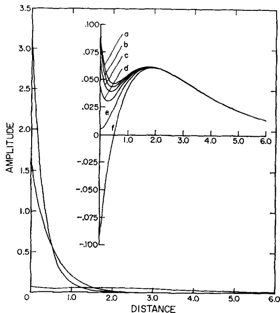
FIG. 1. Orbitals for the 2^2S state of Li. The large drawing is of the SOGI orbitals ( \bar{Z}=0.434^\circ ); the core orbitals remain essentially unchanged when \bar{Z} is within 10^\circ of 0. The insert shows the valence orbital for various values of \bar{Z} ; a: \bar{Z}=0 , b: \bar{Z}=0.434^\circ , c: \bar{Z}=1.0^\circ , d: \bar{Z}=2.0^\circ , e: \bar{Z}=4.0^\circ , f: \bar{Z}=10^\circ . Distance is in atomic units.
