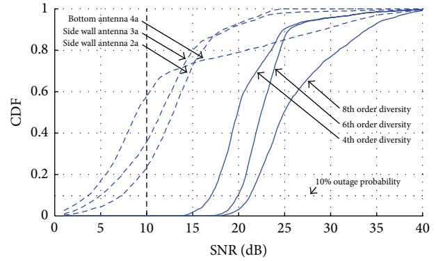
FIGURE 7: Cumulative distribution function (for an x -oriented dipole).
