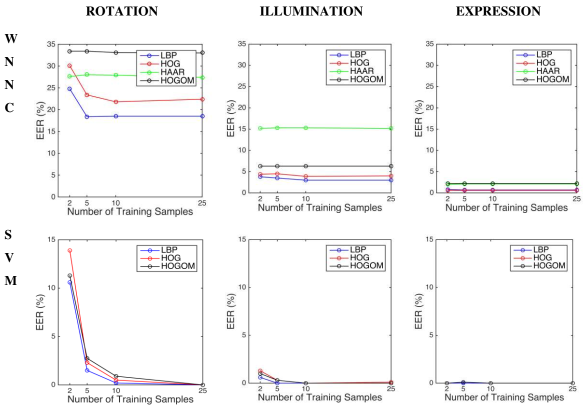
Figure 4. WNNC and SVM Equal Error Rate (EER) when trained with all modalities.
