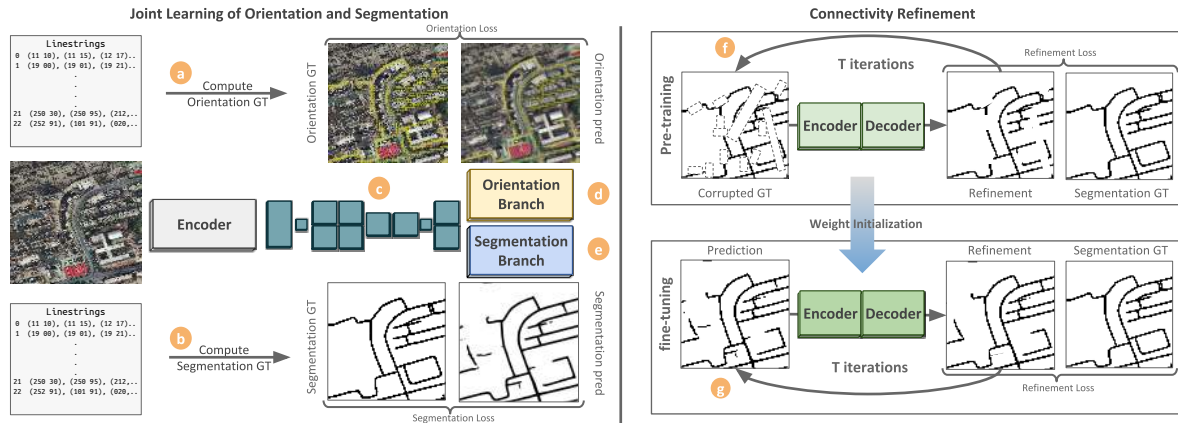
Figure 2: Our approach for extracting connected road topology from satellite images. Annotations in the form of line strings, are converted to (a) orientation groundtruth and (b) road groundtruth masks. We use encoder-decoder structure with (c) stacked multi-branch module to jointly learn (d) orientation and (e) segmentation, providing dual supervision to the model. The orientation task is designed to improve the road connectivity. Finally, a connectivity refinement network, (f) pre-trained with corrupted groundtruths to remove false roads and further improve the road connectivity, is (g) fine-tuned with road segmentation output to iteratively enhance the estimated road networks.
