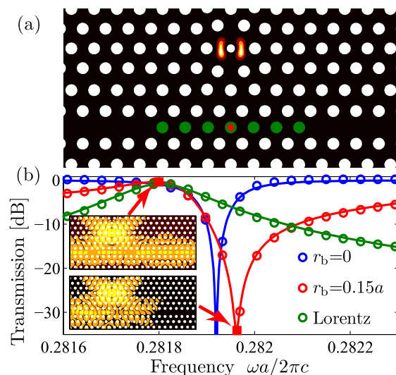
Fig. 1. (a) Photonic crystal waveguide-cavity structure with holes of radii r_b in the waveguide (red and green) and r_0 in the remaining lattice. The field profile |H|^2 is overlaid. (b) Transmission spectra found from 3D FDTD calculations (circles) for the different blockade configurations in (a), where a is the lattice constant and c the speed of light. The blue curve corresponds to an unblocked waveguide, and the red and green curves match the colors in (a). The solid lines are fits using Eq. (3). The insets show |H|^2 using CW excitation in the “on” and “off” states of the Fano structure as indicated by the red squares.
