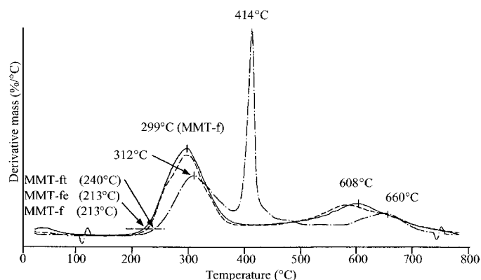
Figure 1. Thermograms of DMDODA-MMT samples MMT-f, MMT-fe and MMT-ft. Peaks above 500^\circ\text{C} represent the decomposition of aromatized pre-char formed from degradation of the DMDODA and dehydroxylation of MMT. Note the initial degradation temperature is \sim 27^\circ\text{C} higher in the THF extracted organoclay.
