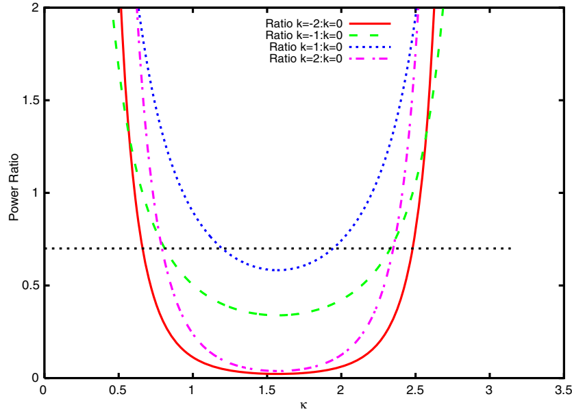
Figure 1. Power in k \neq 0 sidebands relative to power in k = 0 sideband for challenge source 1B.3.2. The true parameters were \lambda = 1.44 , \kappa = 1.295 . Our estimated inclination was \kappa = 1.262 .
