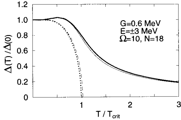
FIG. 6. Pairing gap (normalized to its value at zero temperature) as a function of temperature (normalized to T_c ) obtained using the parameter set (i), see text, at N = 18 . The notations for the modified gap \bar{\Delta}(T) and the usual finite-temperature BCS gap \Delta(T) are the same as in Fig. 5. The corresponding values of these gaps but obtained without the correction -G\bar{v}_j^2 and -Gv_j^2 are shown by thin solid and dashed lines, respectively.
