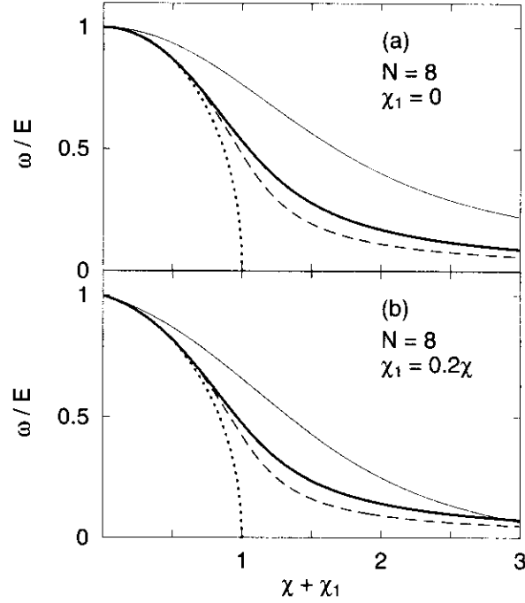
FIG. 1. Normalized excitation energies as a function of the interaction \chi + \chi_1 for N = 8 particles: exact solution, thin solid line; RPA, dots; renormalized RPA, dashes; and modified RPA, thick solid line.
